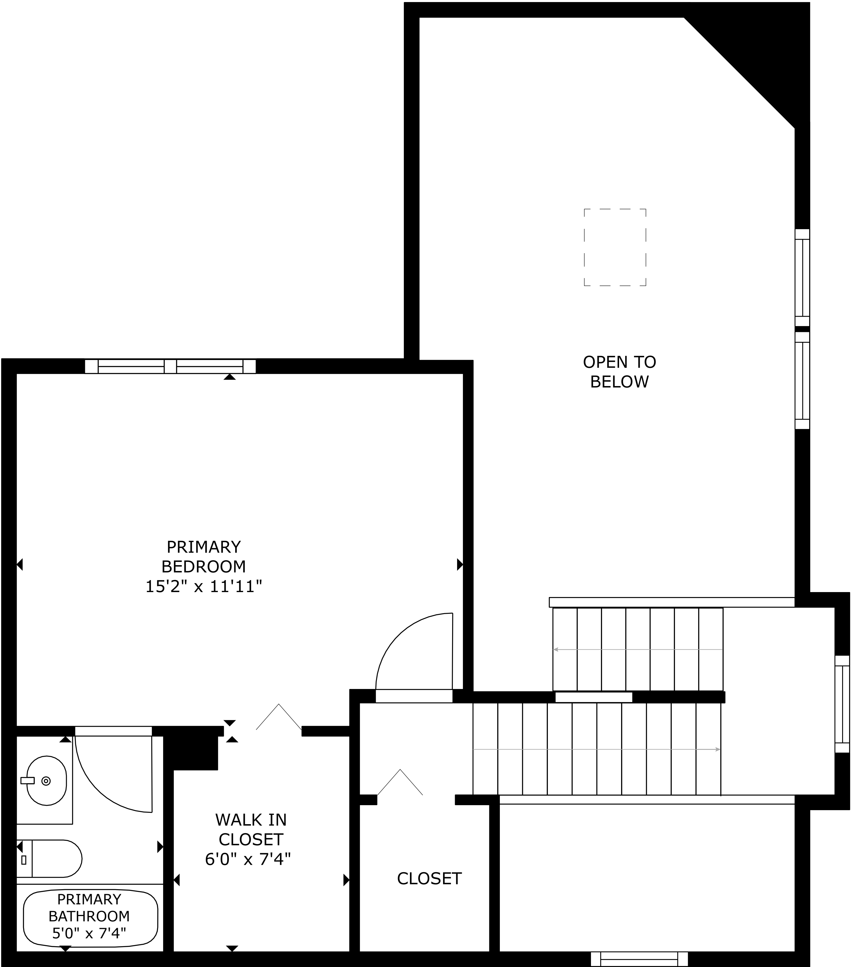
FLOOR 2
