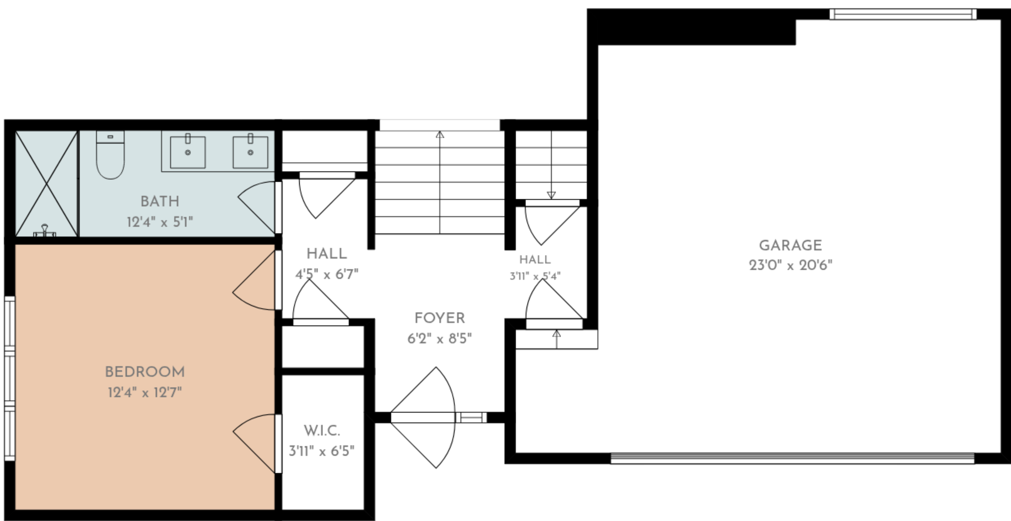
1st floor
