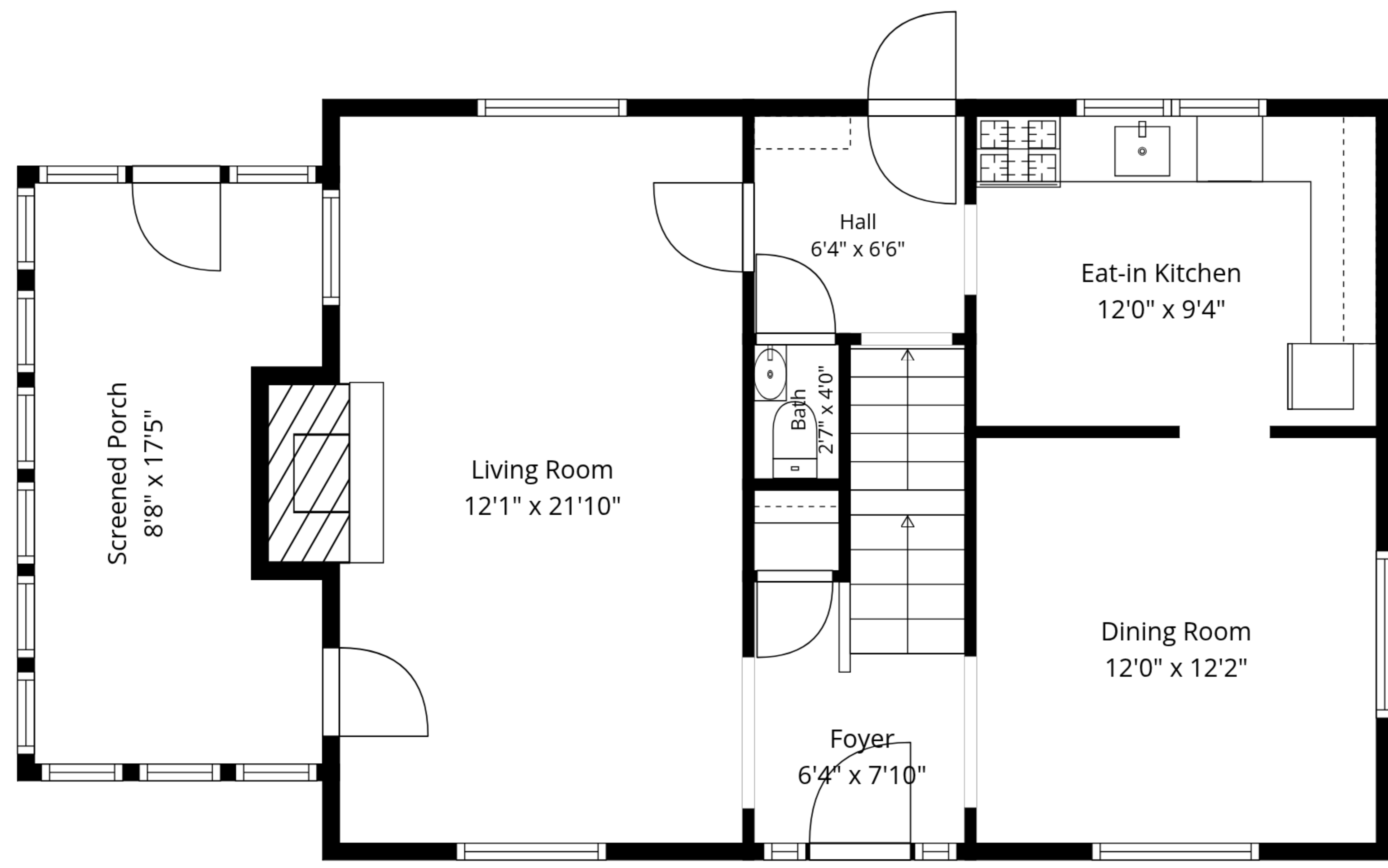
1st Floor
