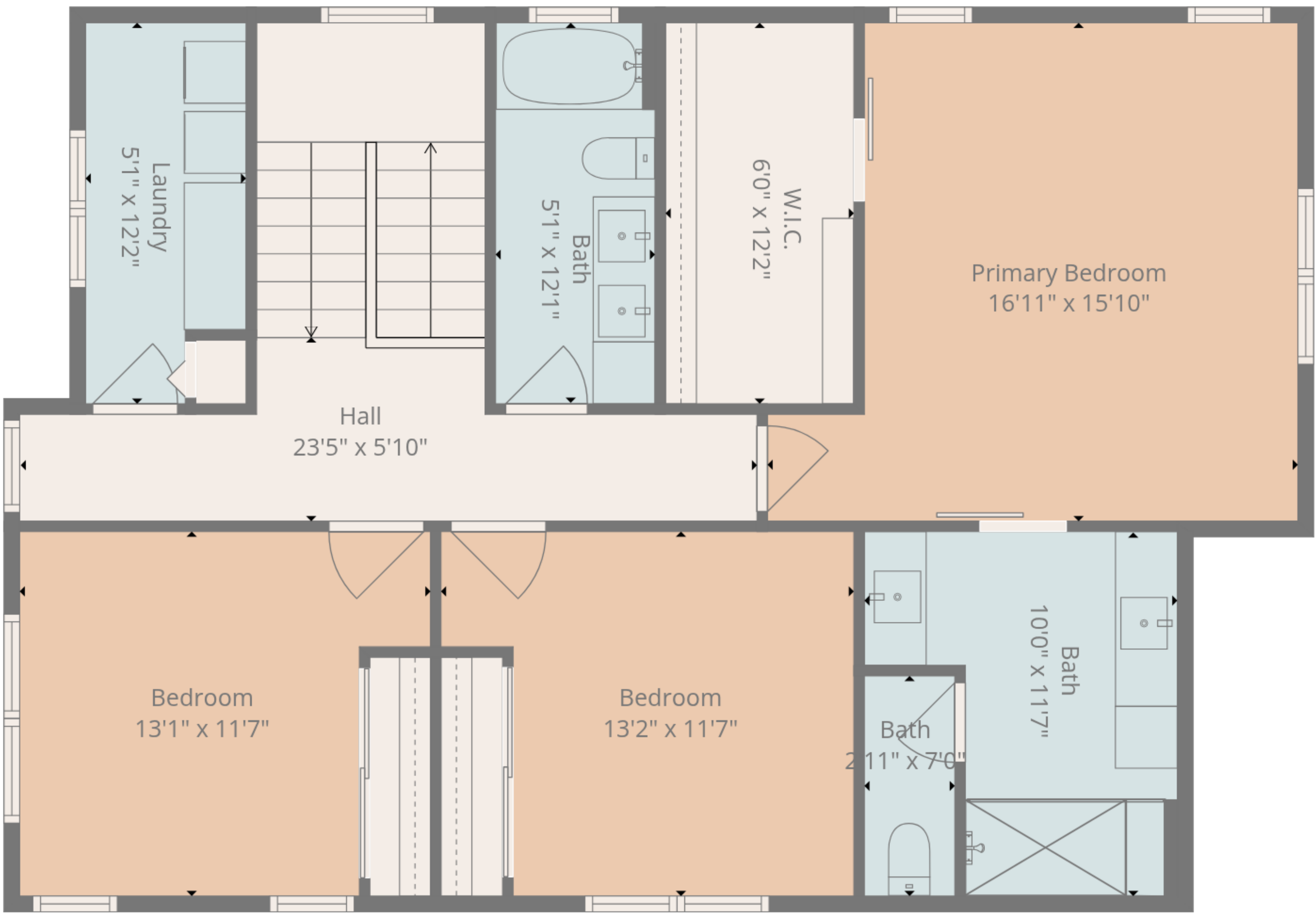
2nd Floor
