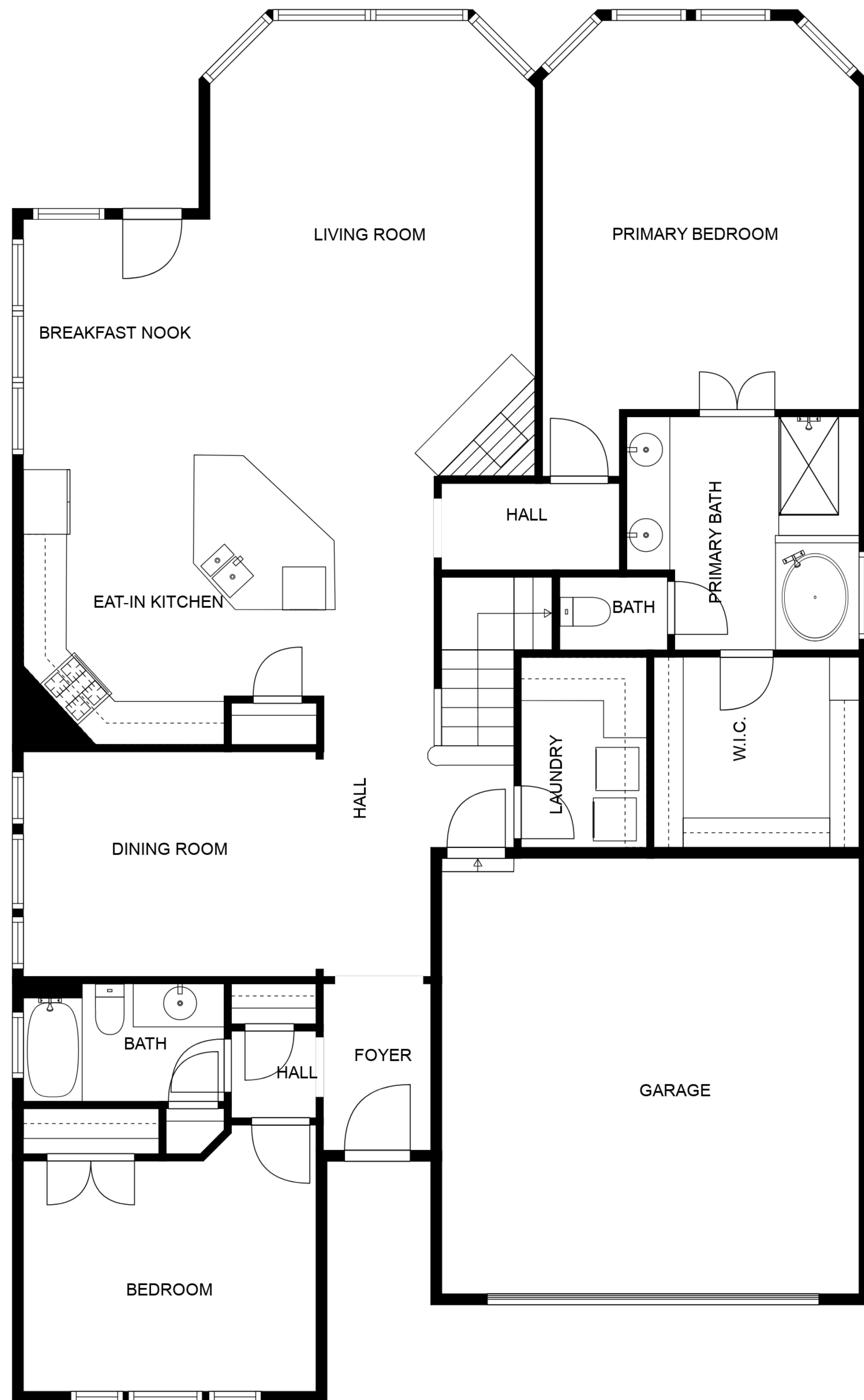
FLOOR 1
