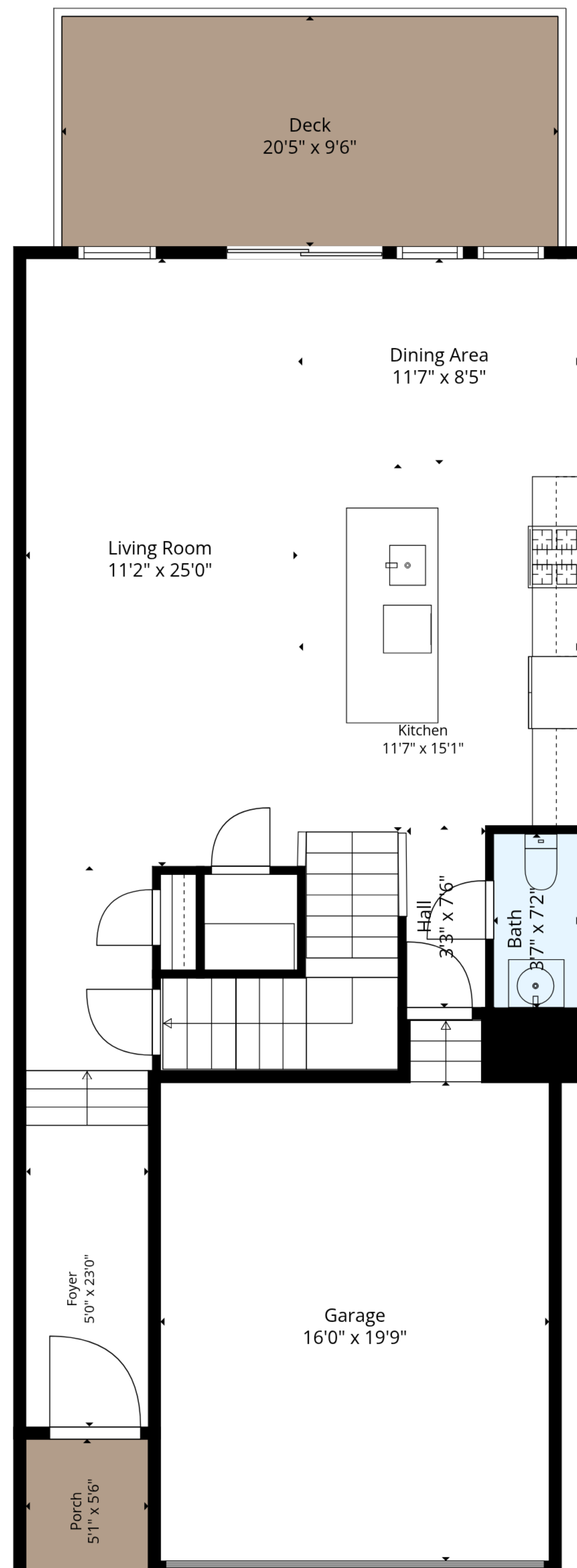
1st Floor
