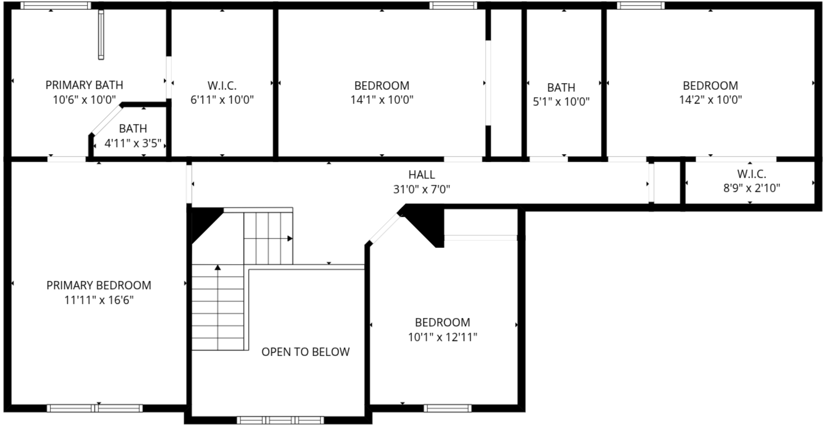
2nd floor
