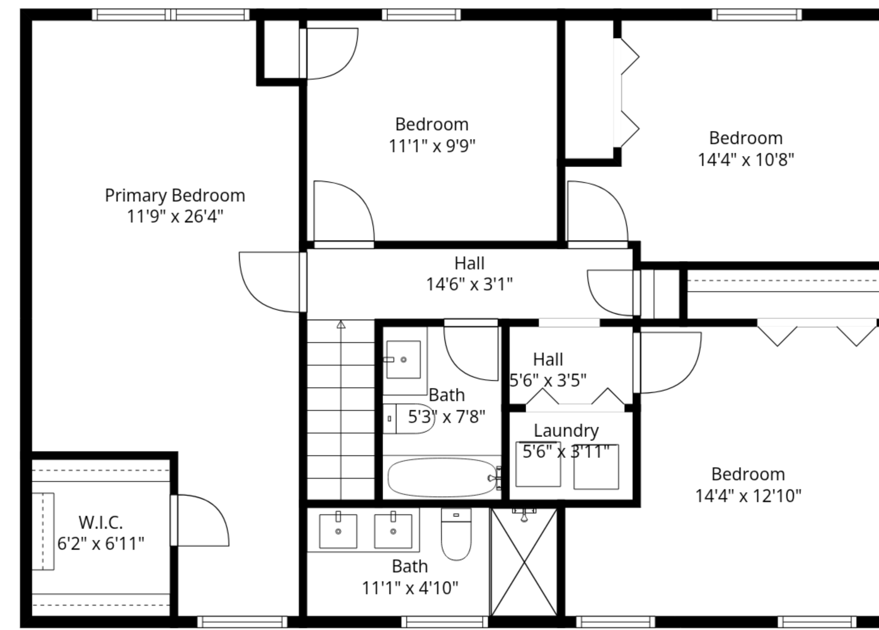
2nd Floor
