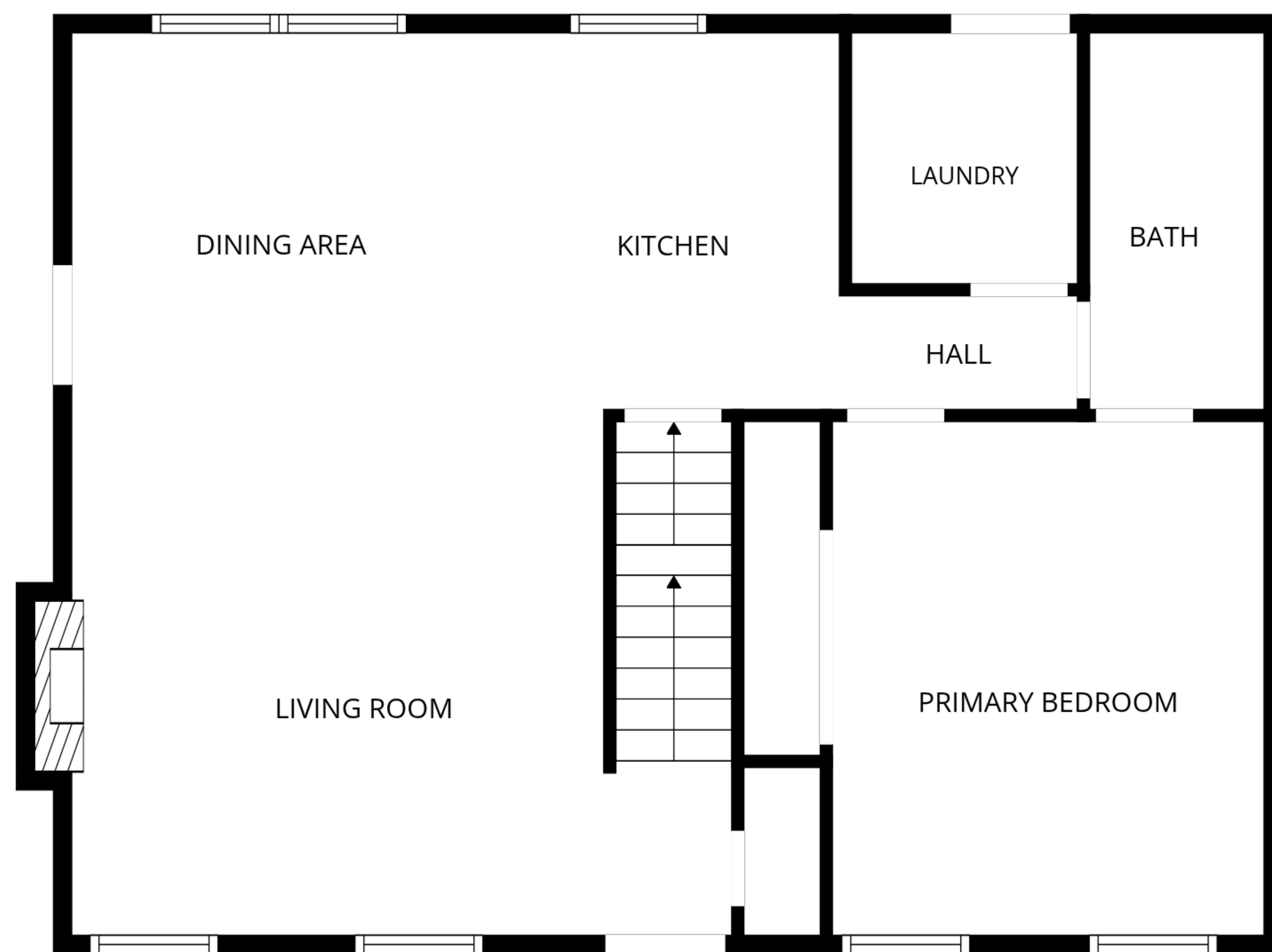
1ST FLOOR
