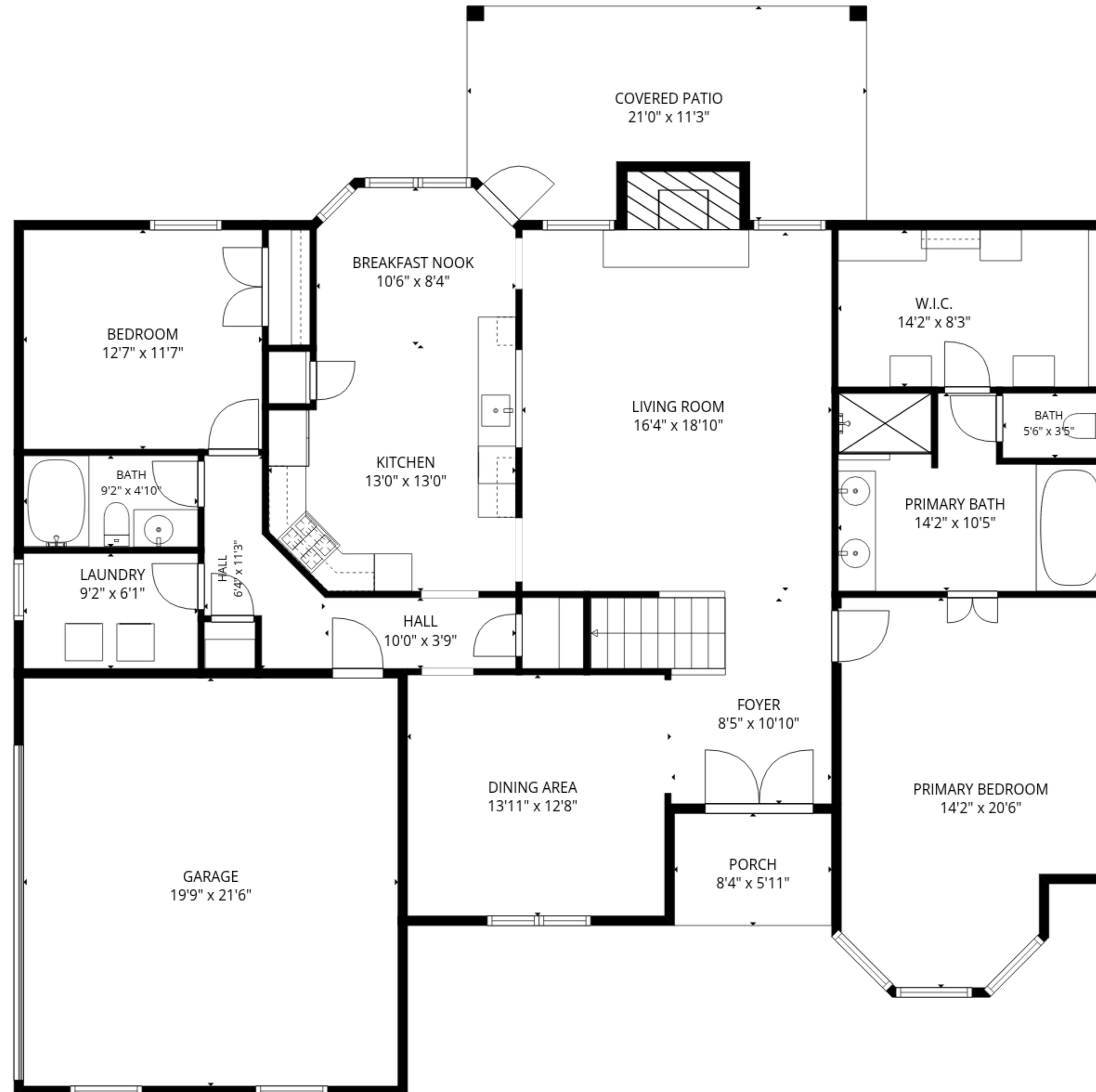
1st floor
