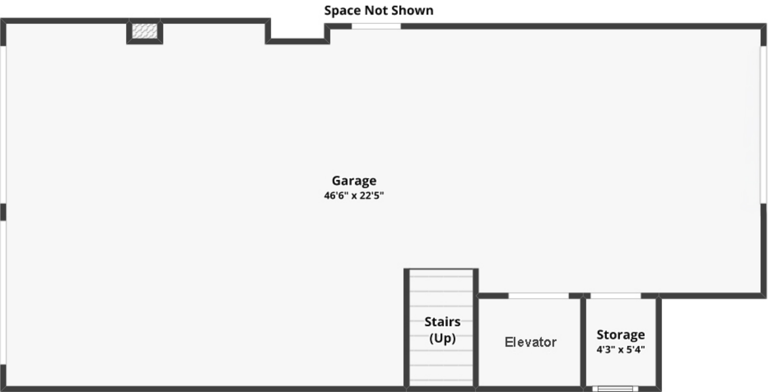
FLOOR 1
