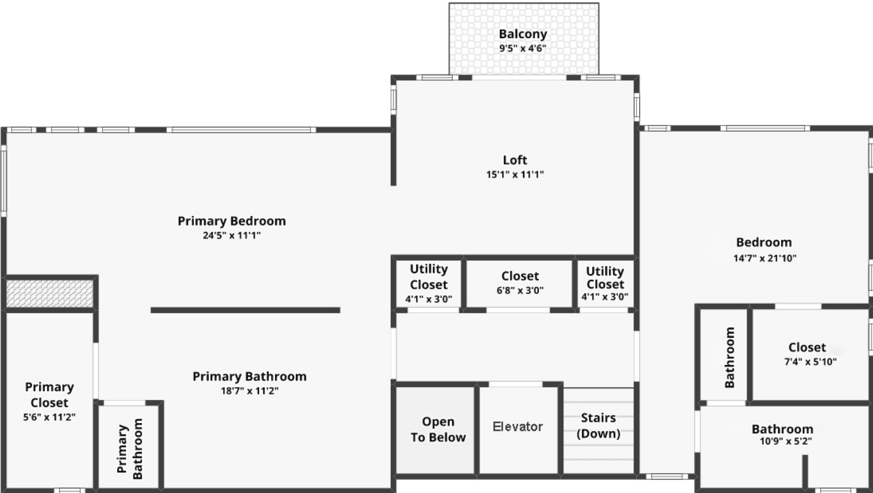
FLOOR 3
