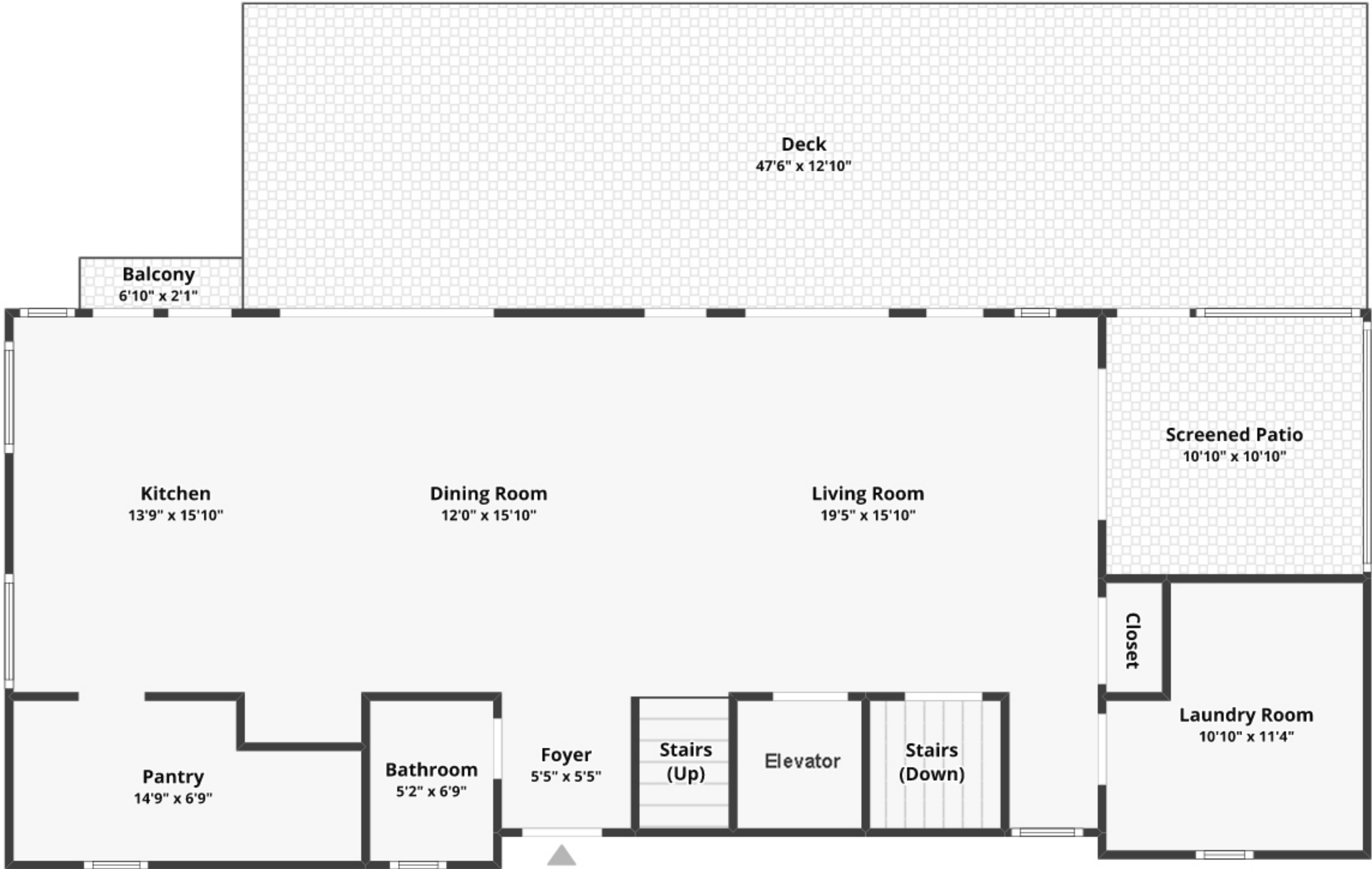
FLOOR 2
