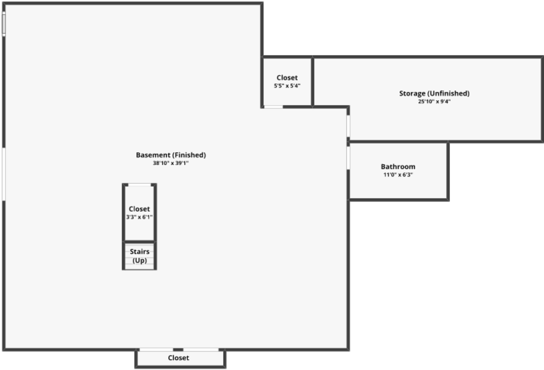
BASEMENT Finished area: ~1,508.08 sq. ft. Unfinished area: ~224.01 sq. ft.
