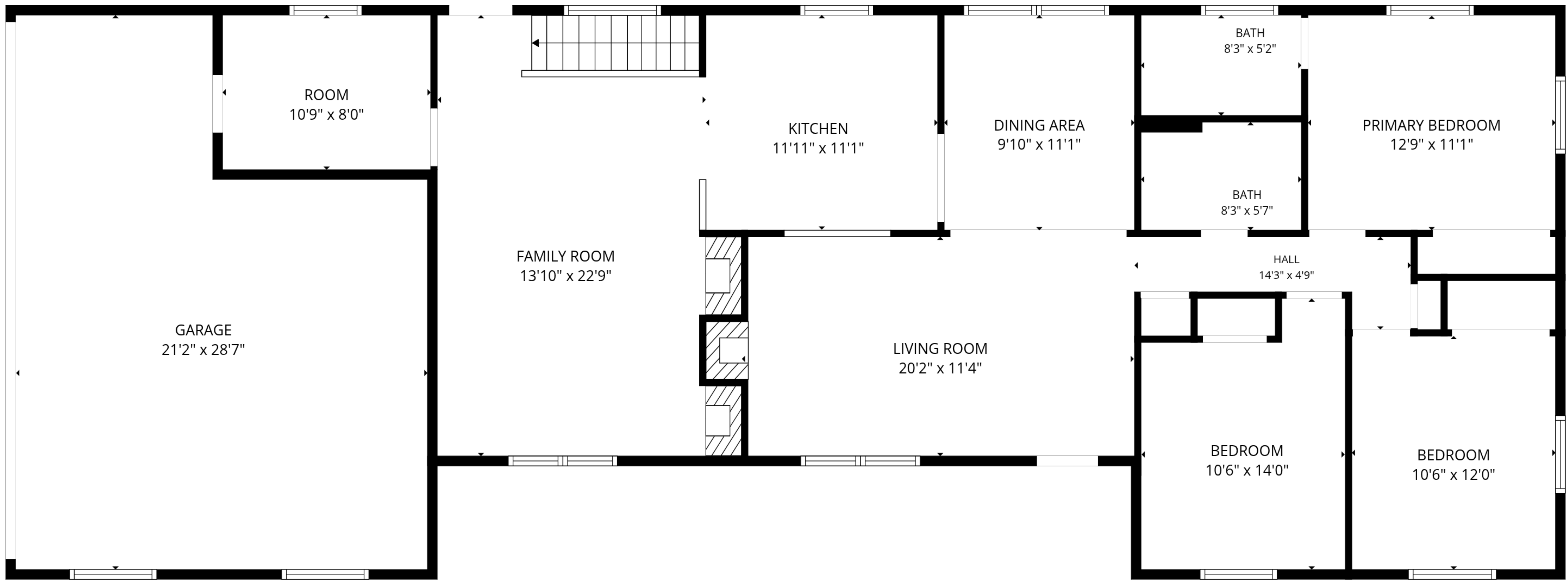
1st floor
