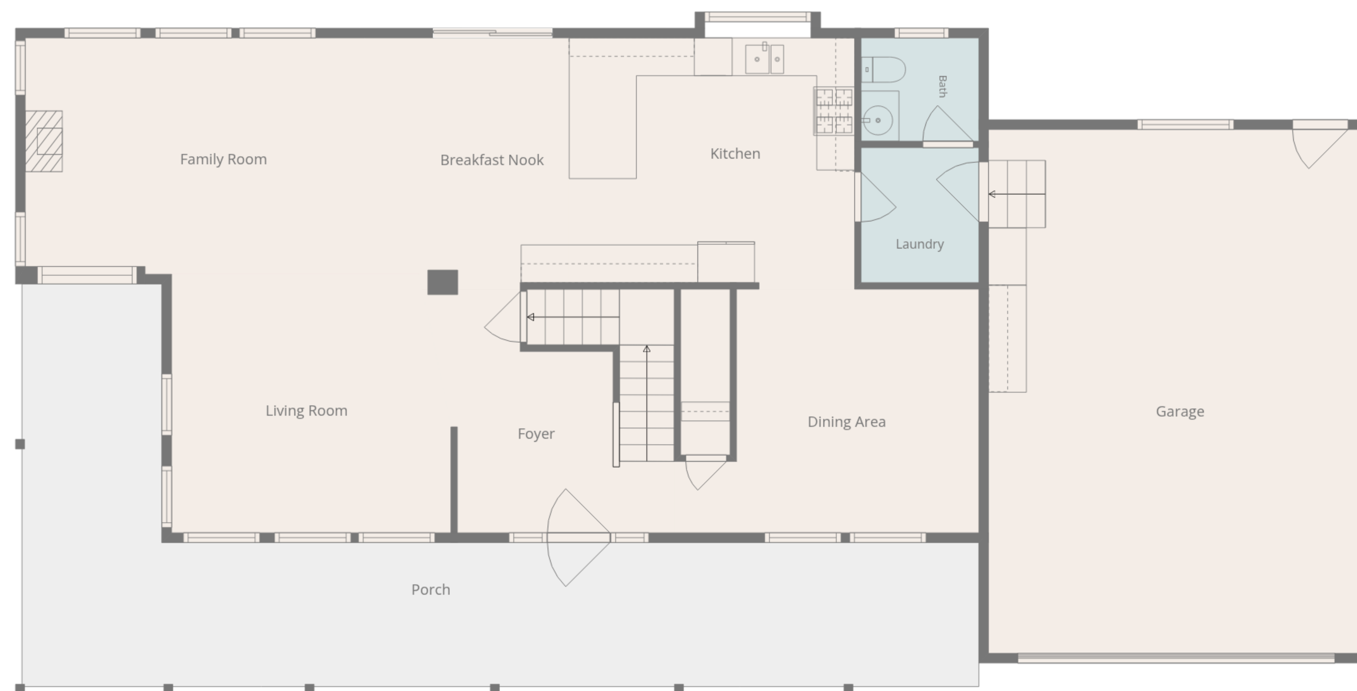
1st Floor
