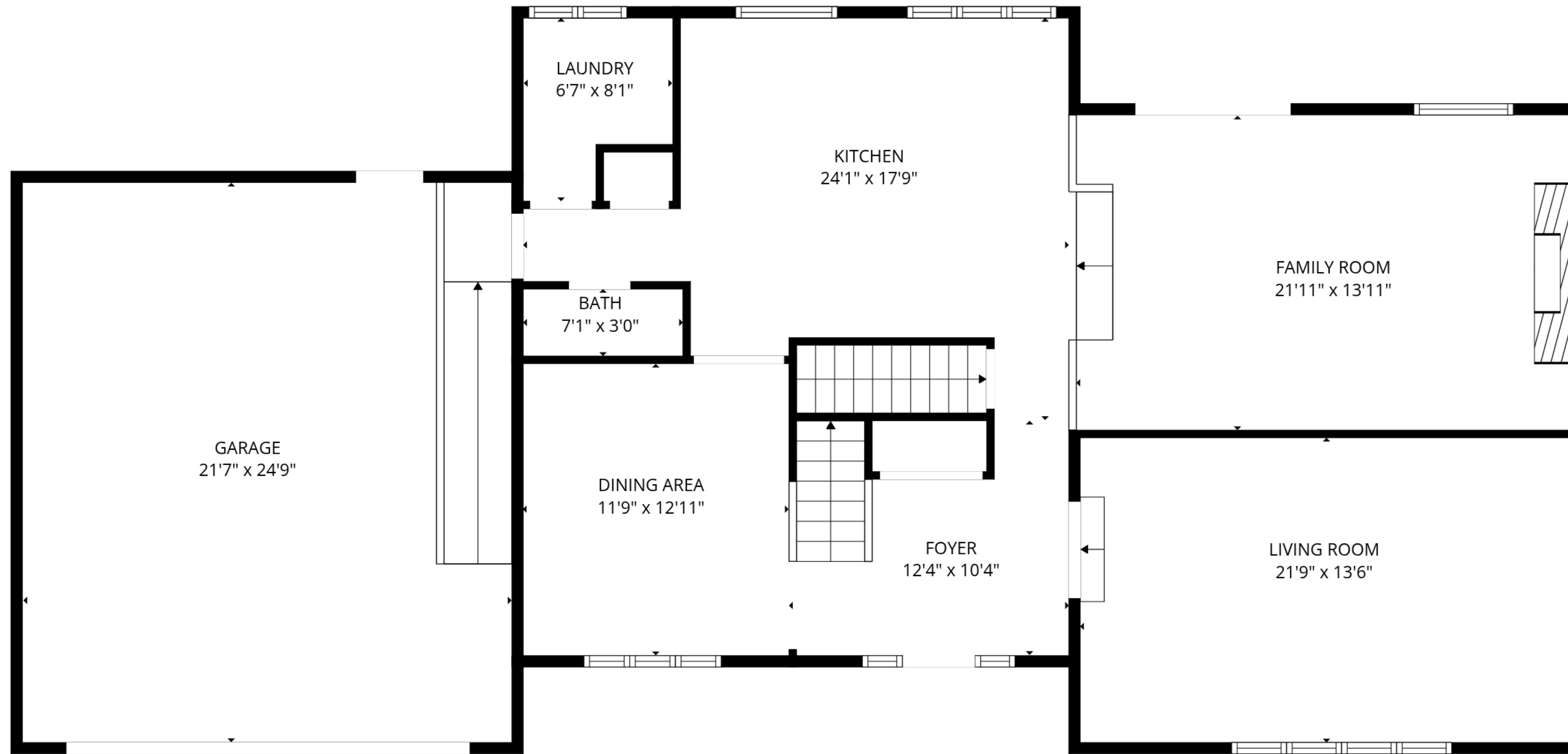
1st floor
