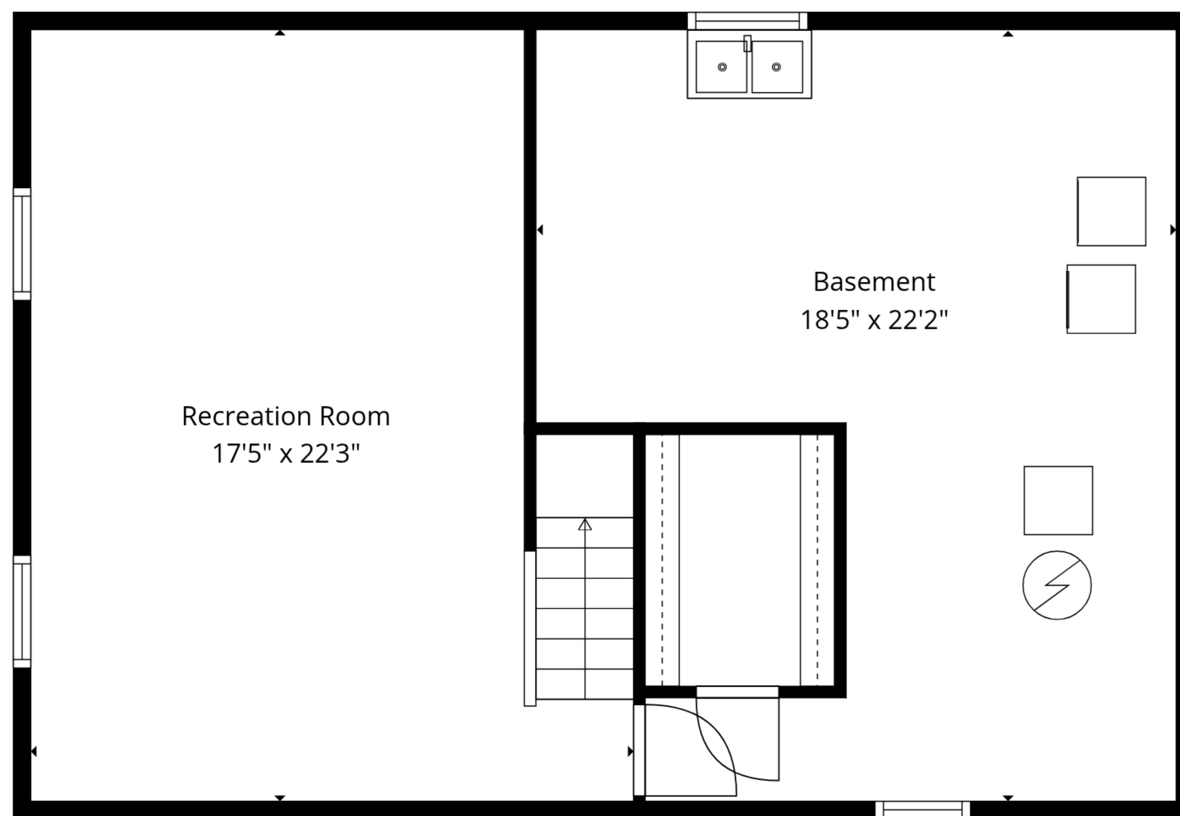
Basement
