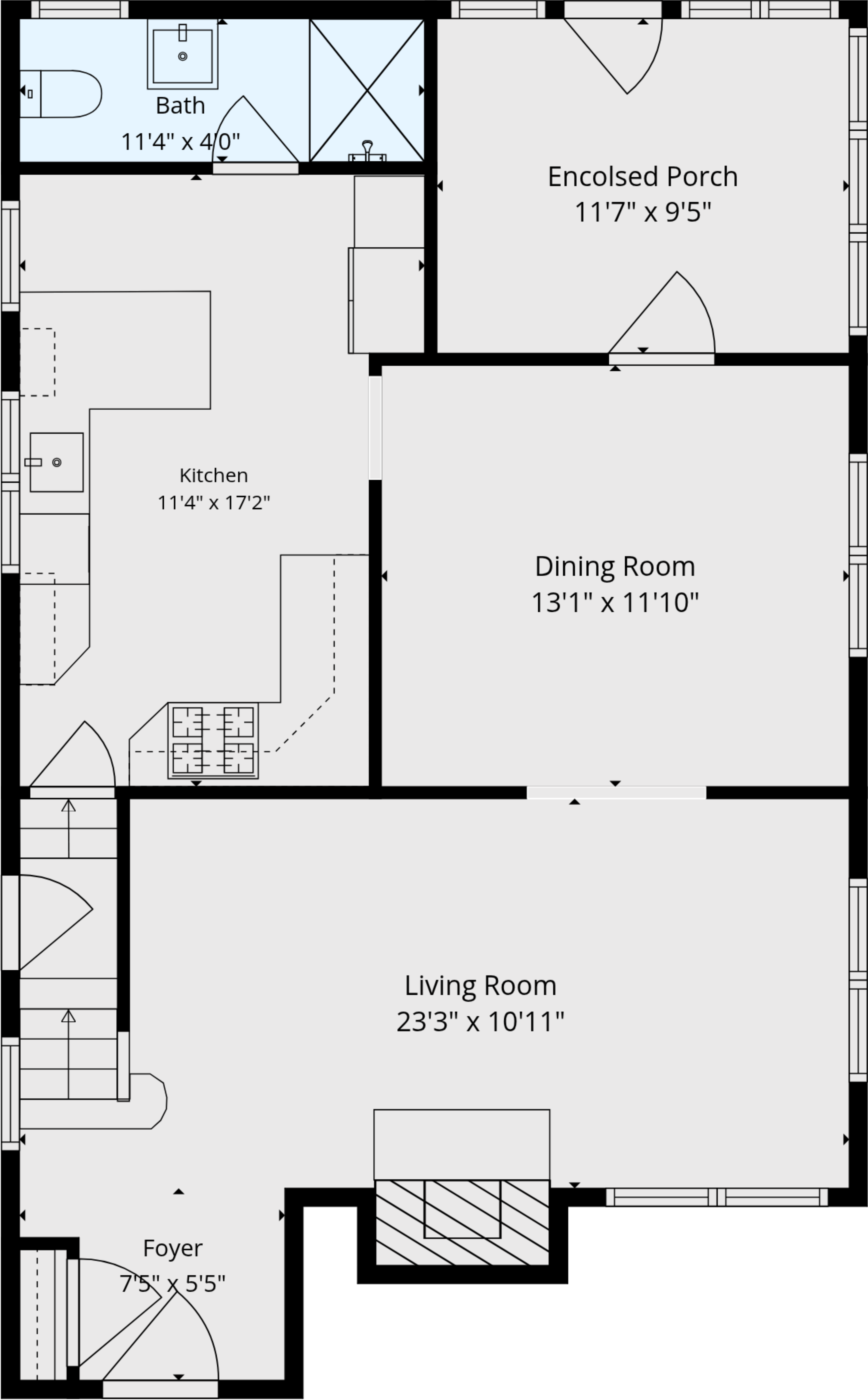
1st Floor
