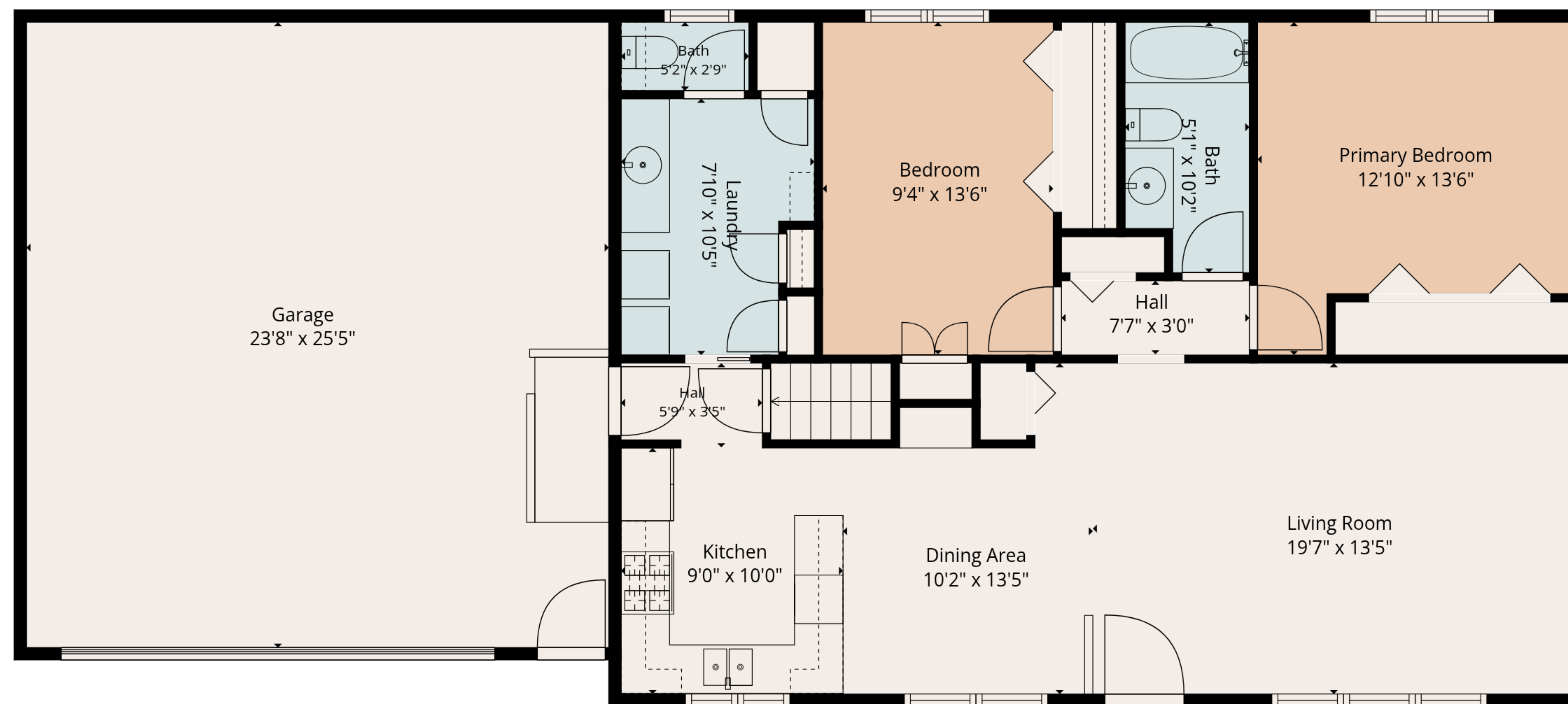
1st Floor
