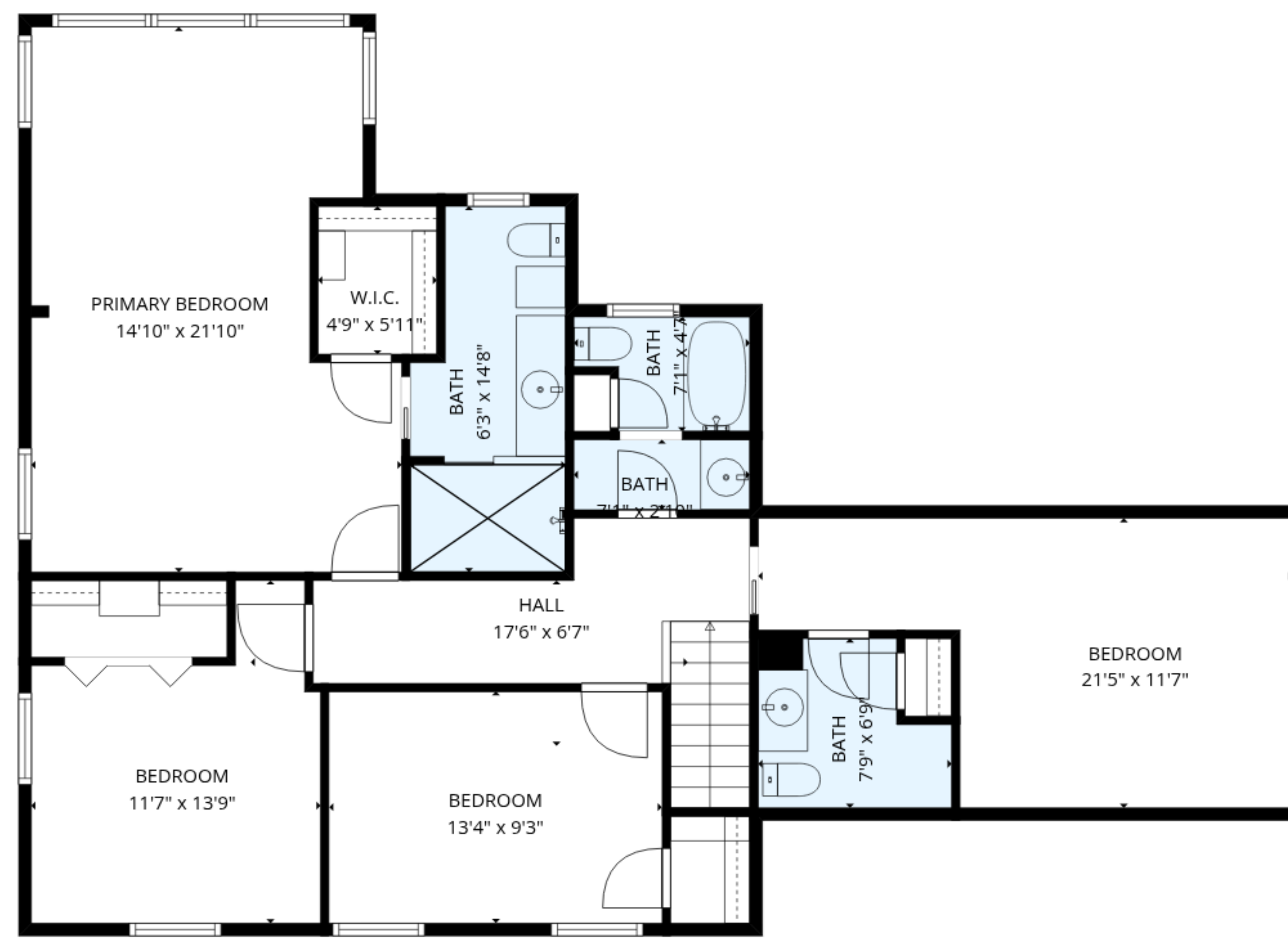
2nd floor
