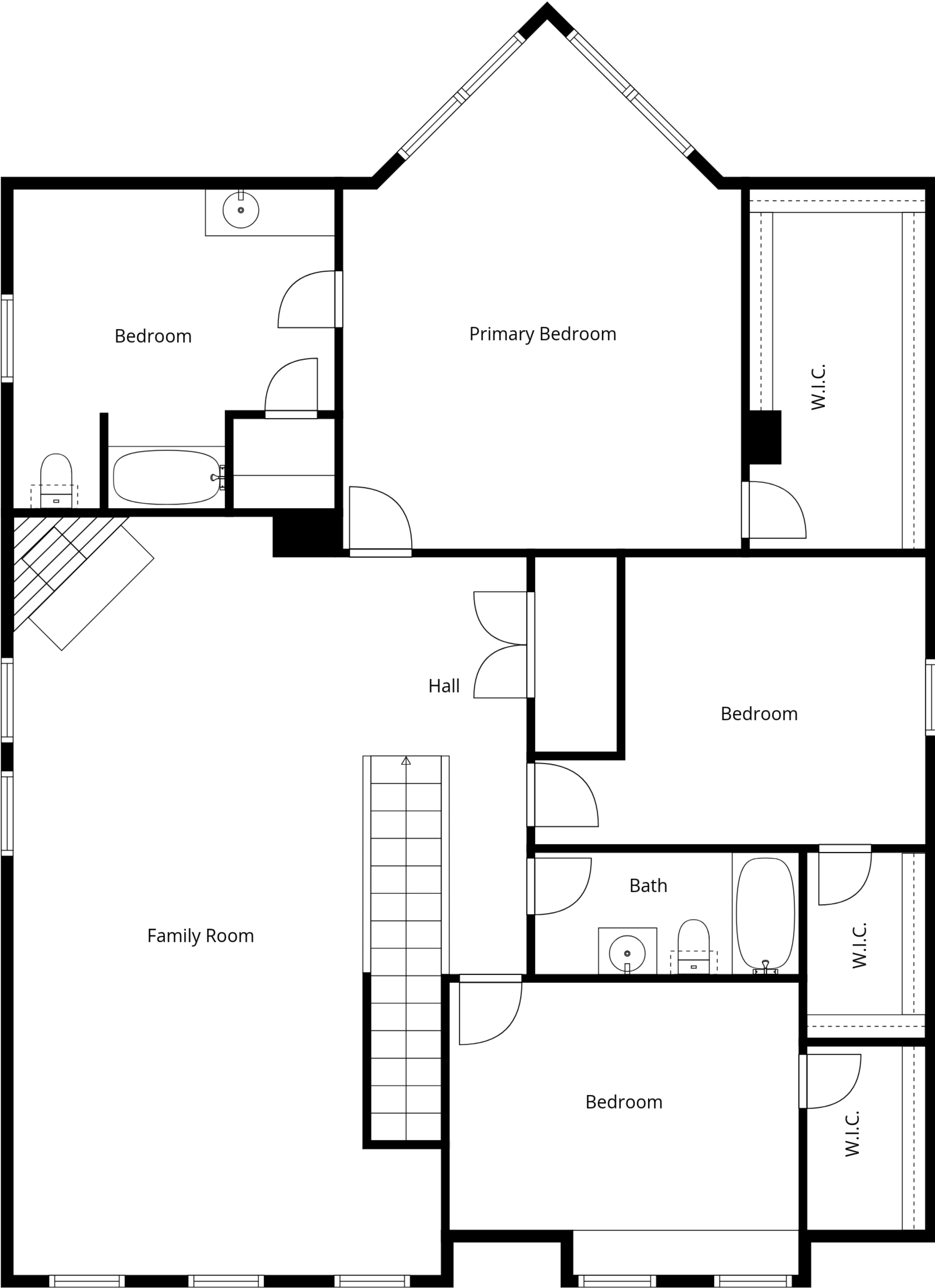
2nd Floor
