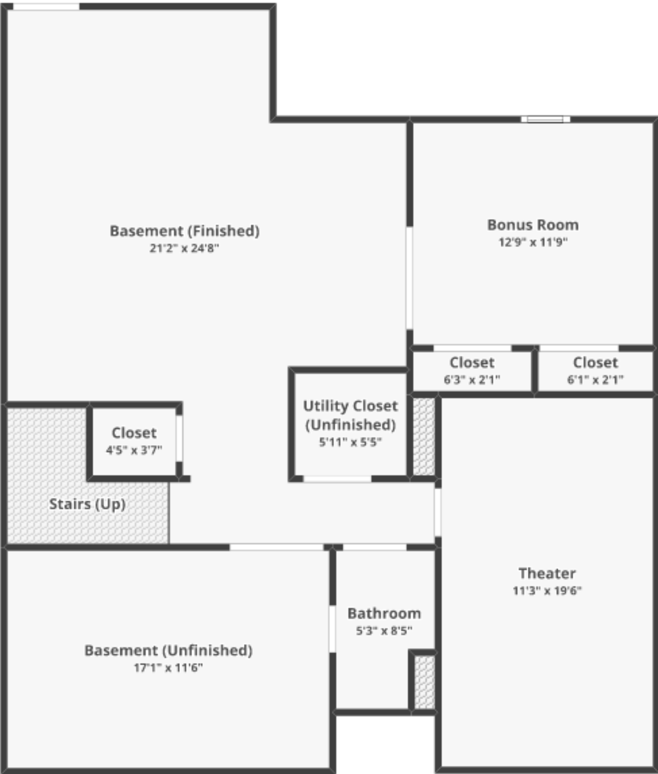
BASEMENT Finished area: ~903.84 sq. ft.
