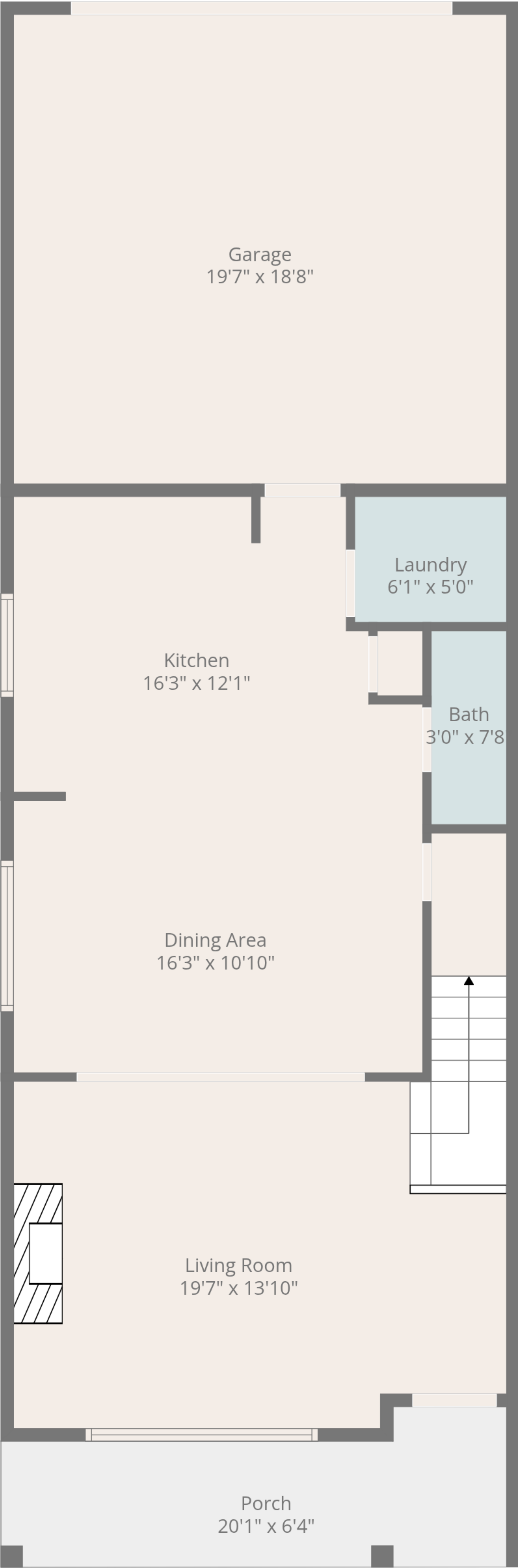
Floor 1
