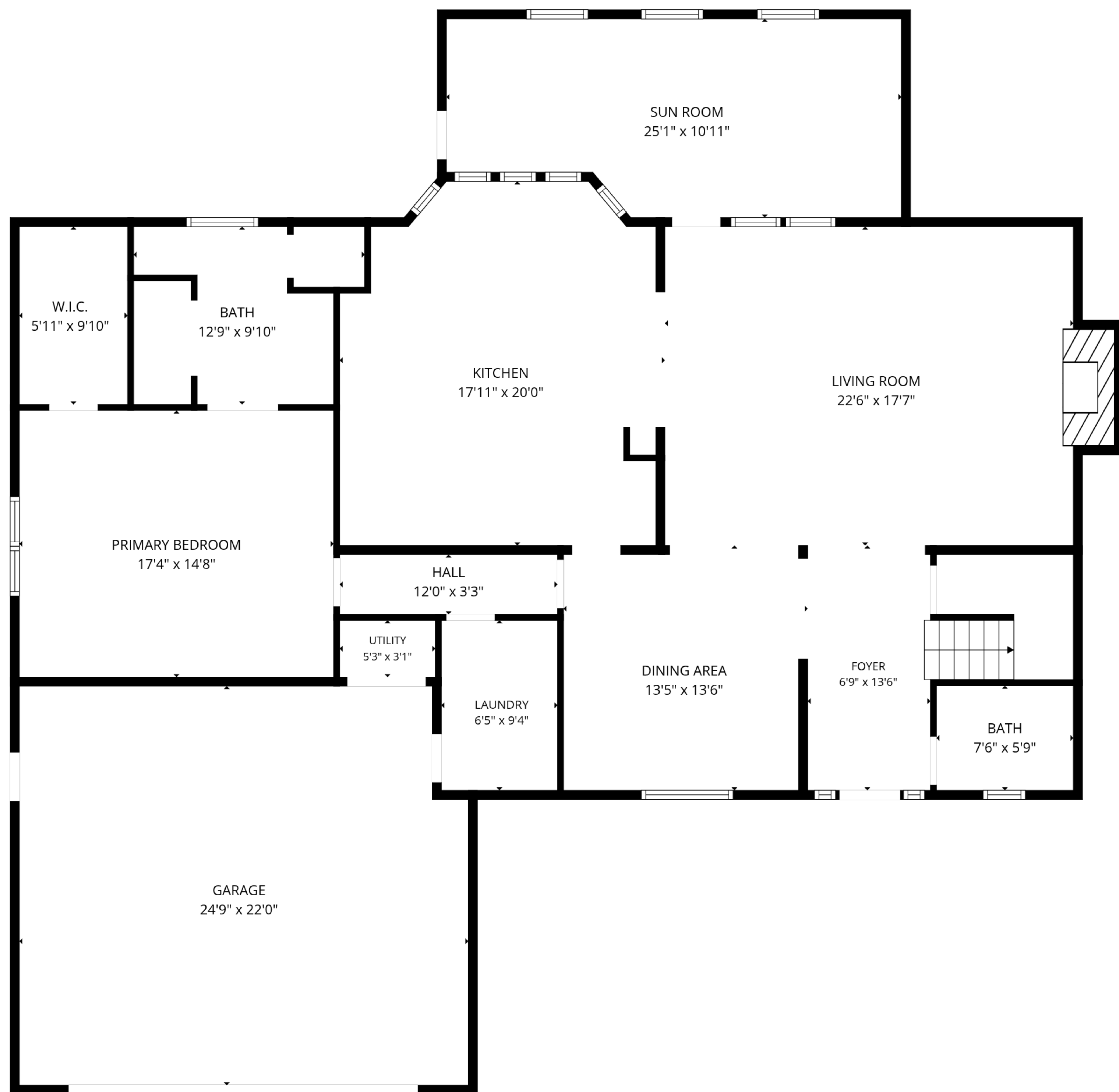
1st floor
