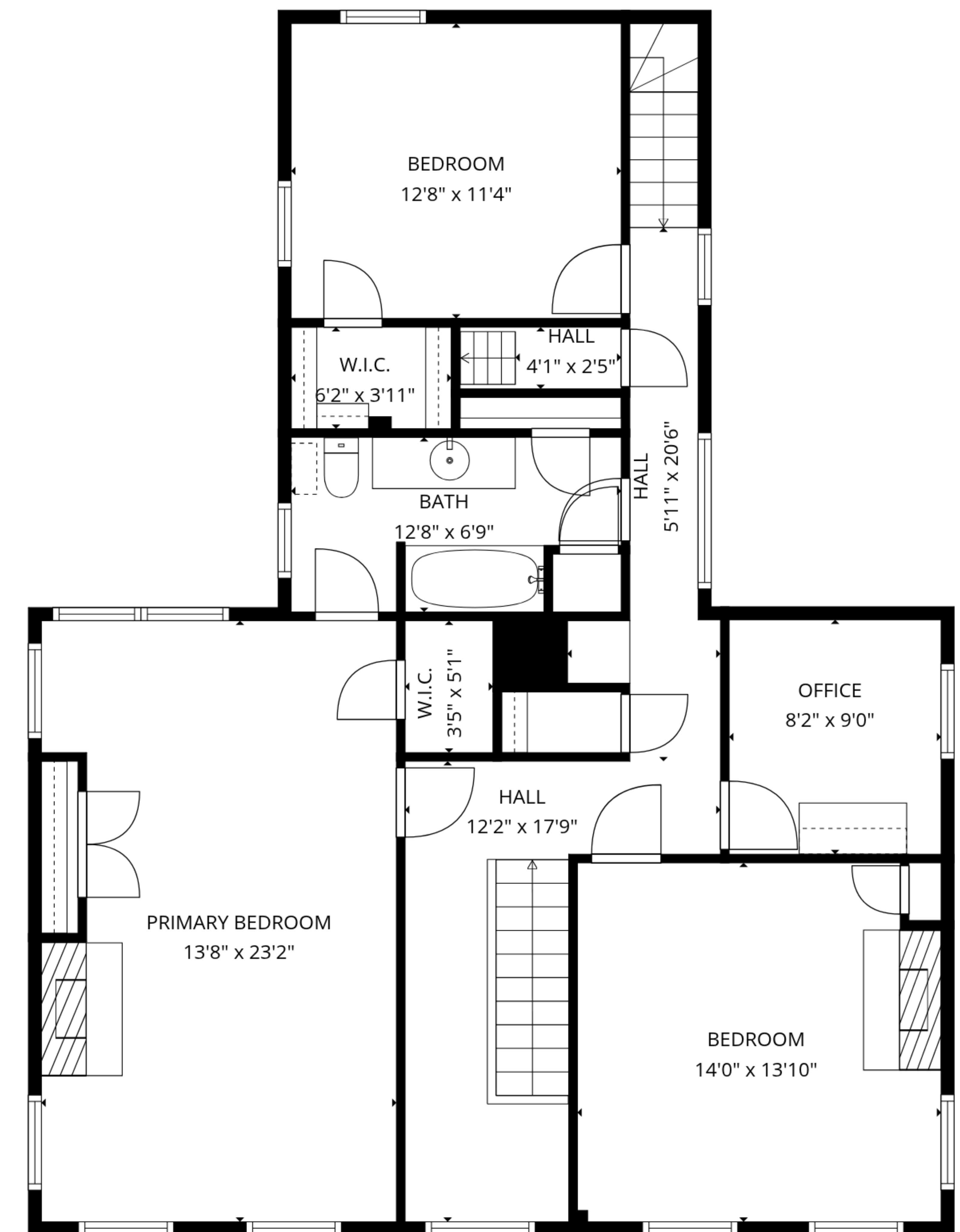
2nd floor
