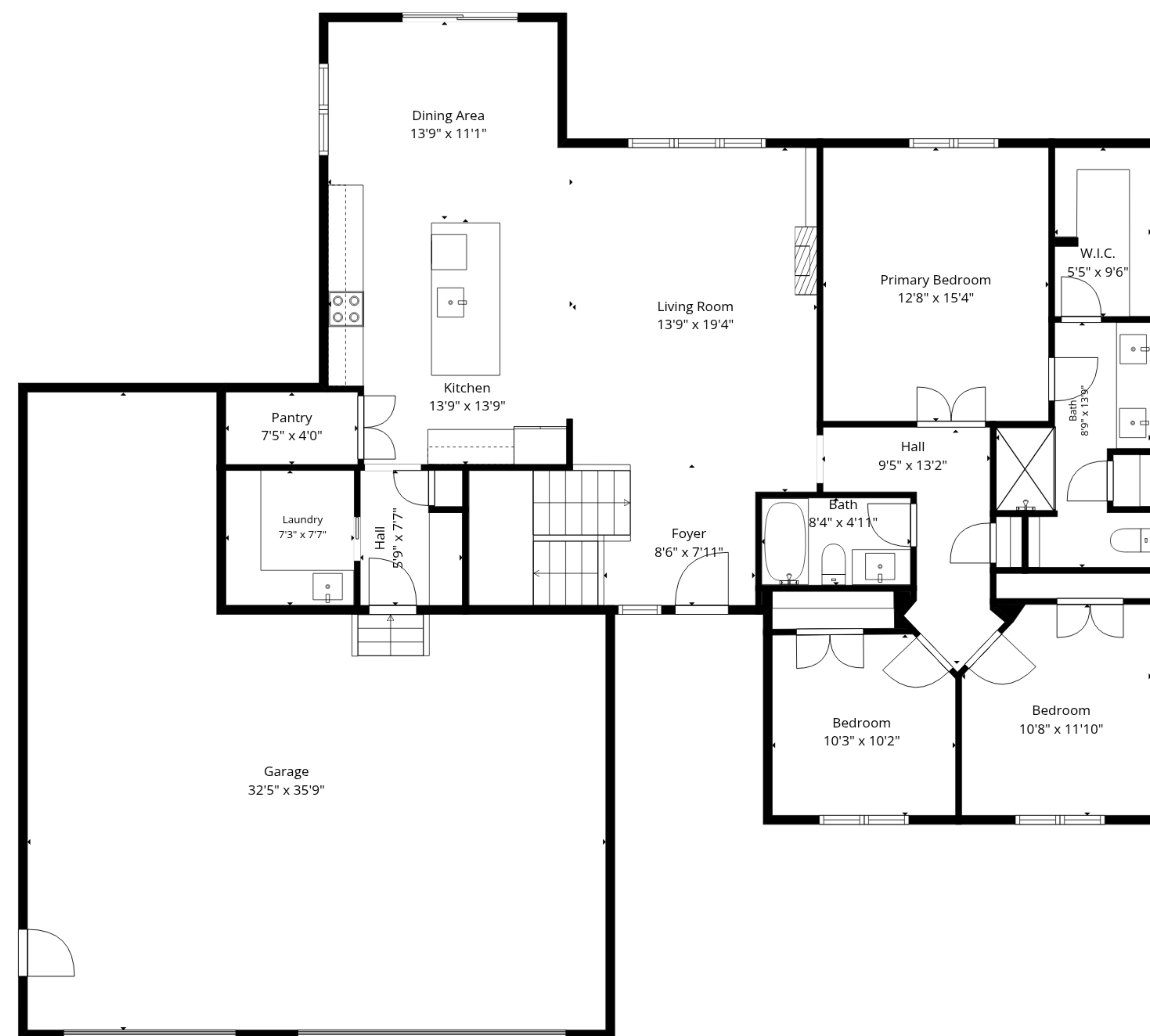
1st Floor
