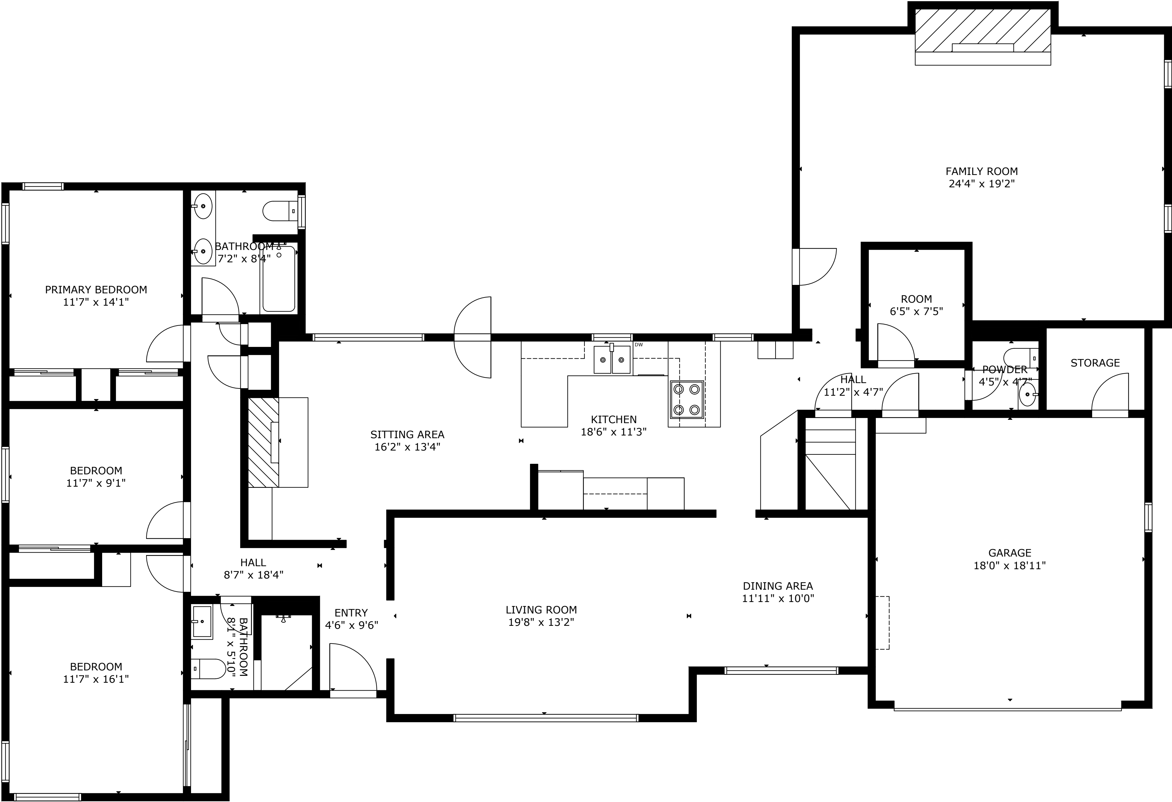
MAIN FLOOR
