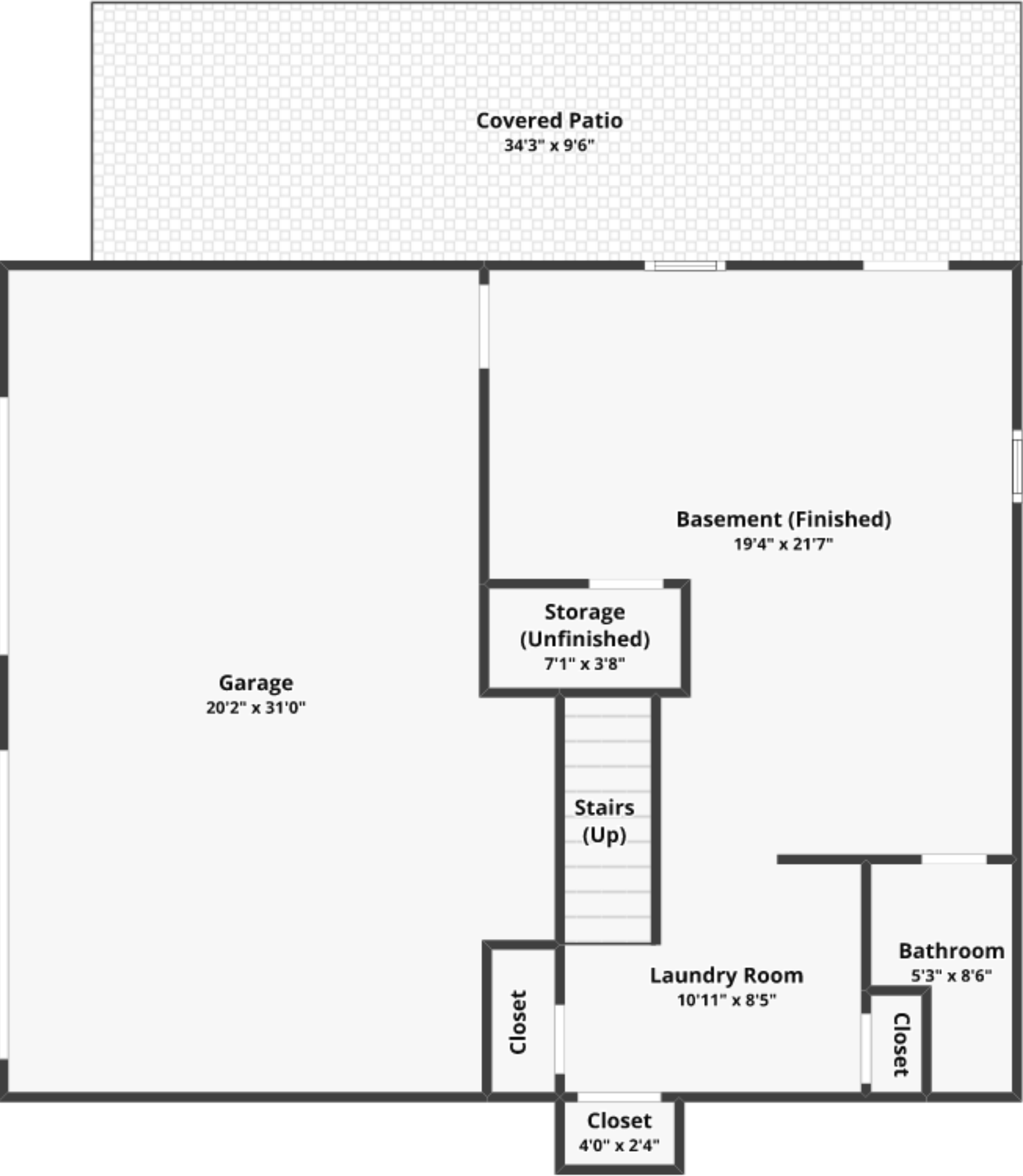
BASEMENT Finished area: ~494.41 sq. ft.
