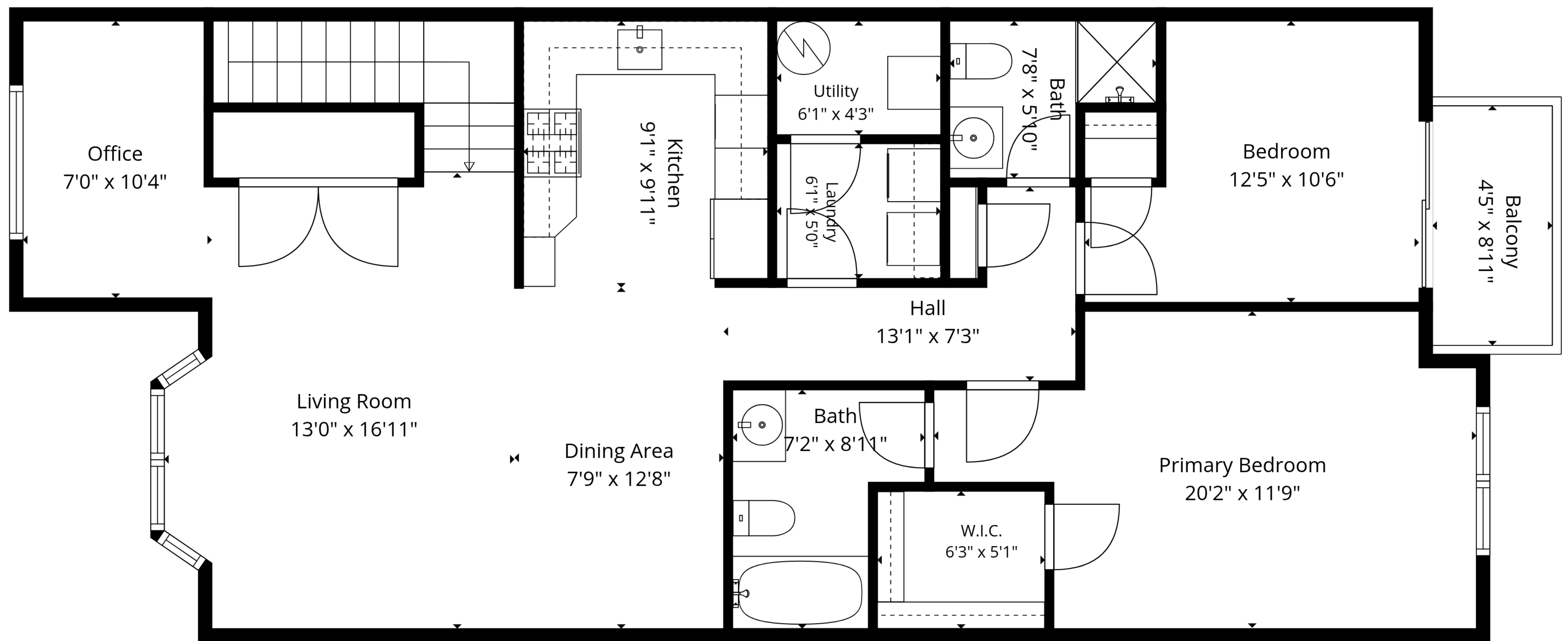
2nd Floor
