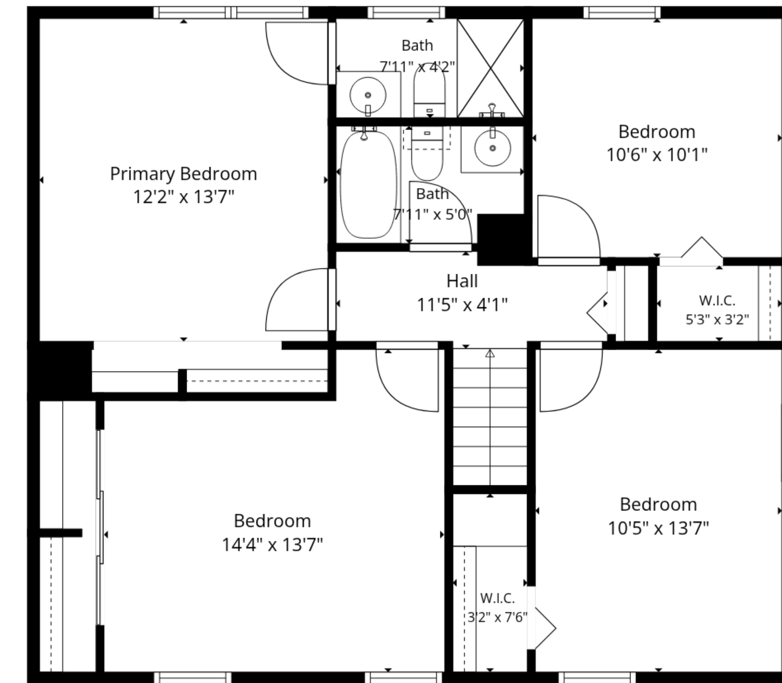
2nd Floor
