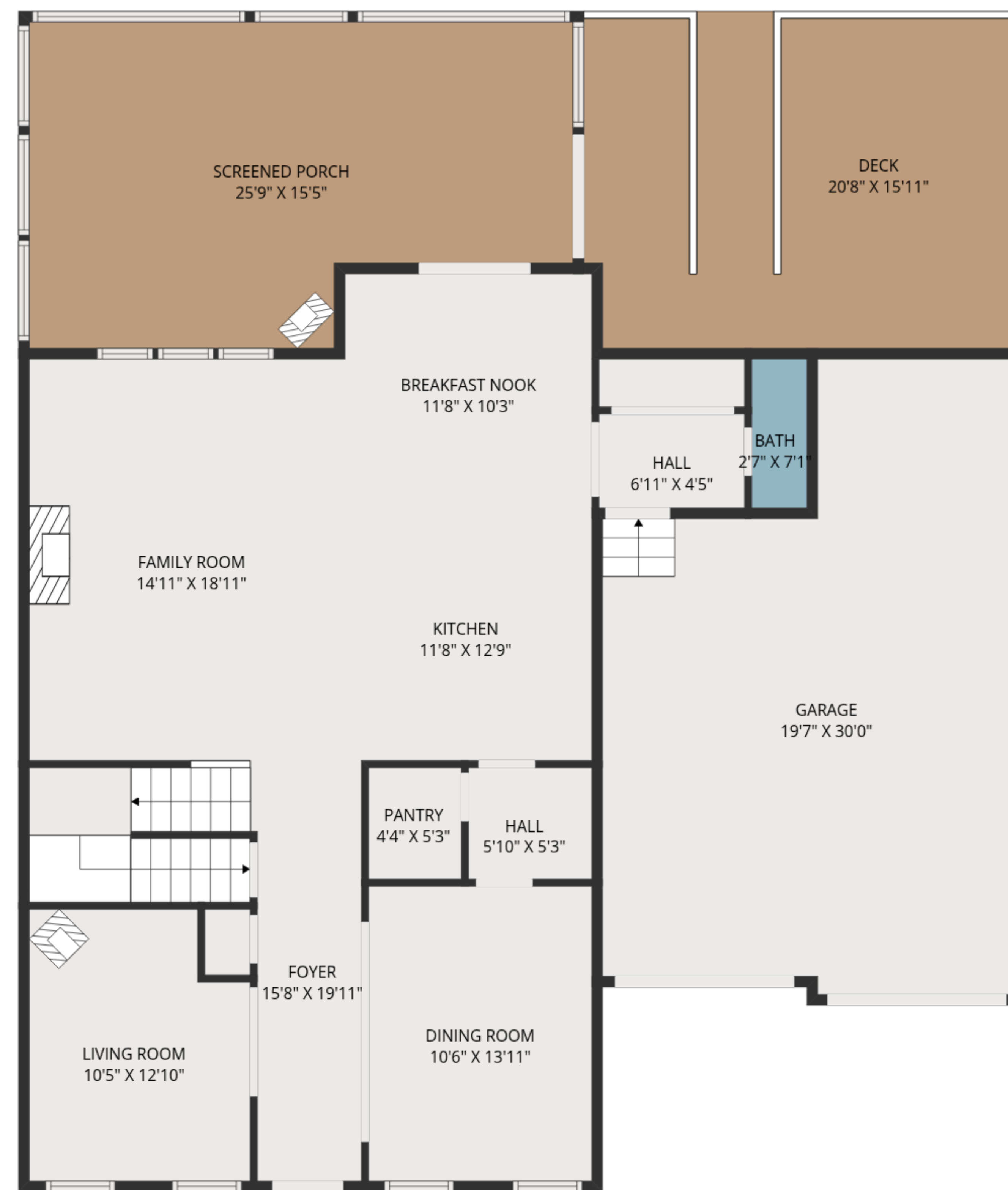
1ST FLOOR
