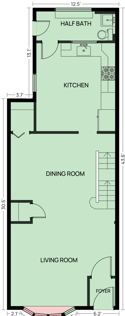
FIRST FLOOR Above grade · 9'7" ceiling · GLA 656 sq ft
