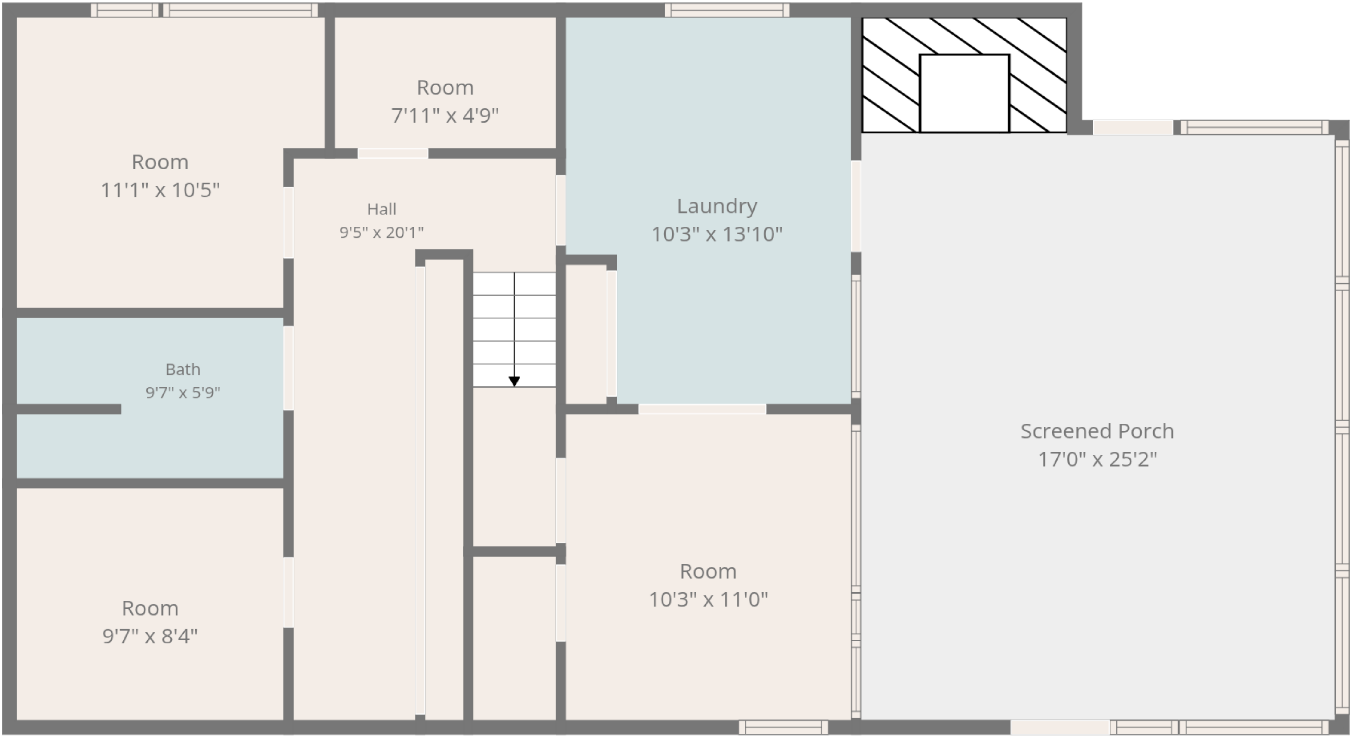
1st Floor
