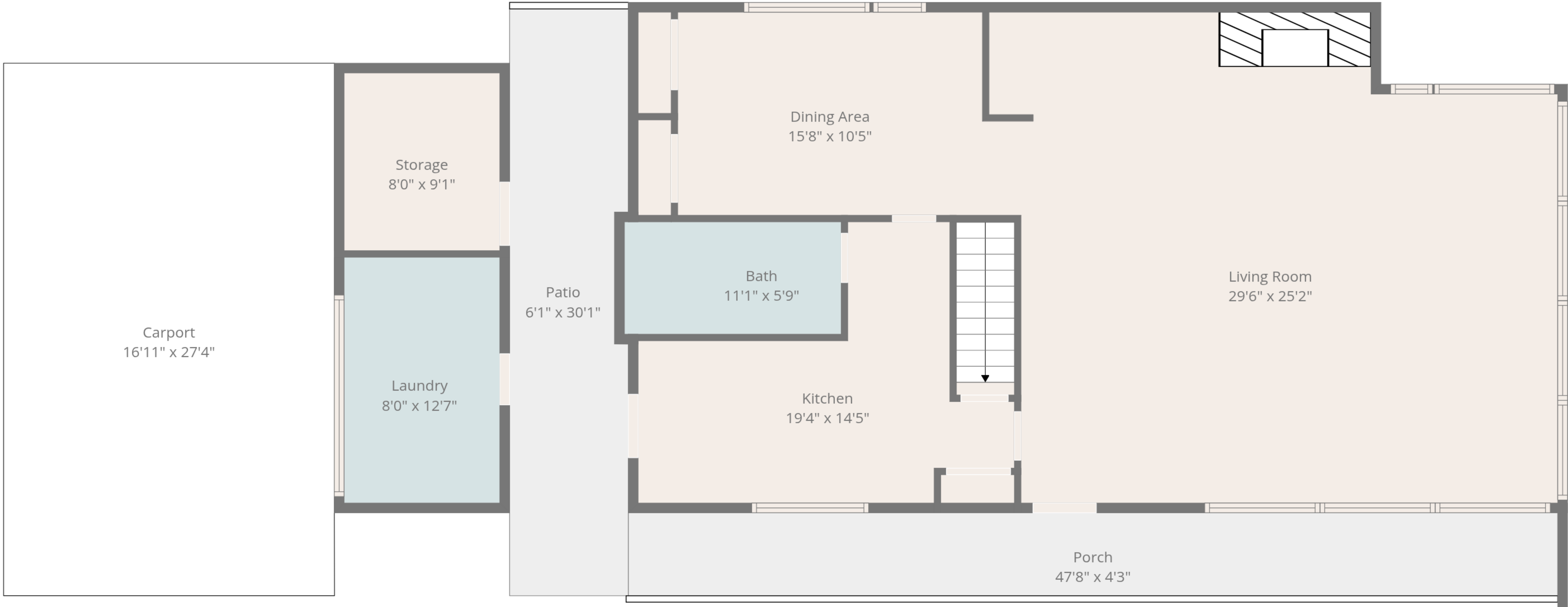
2nd Floor
