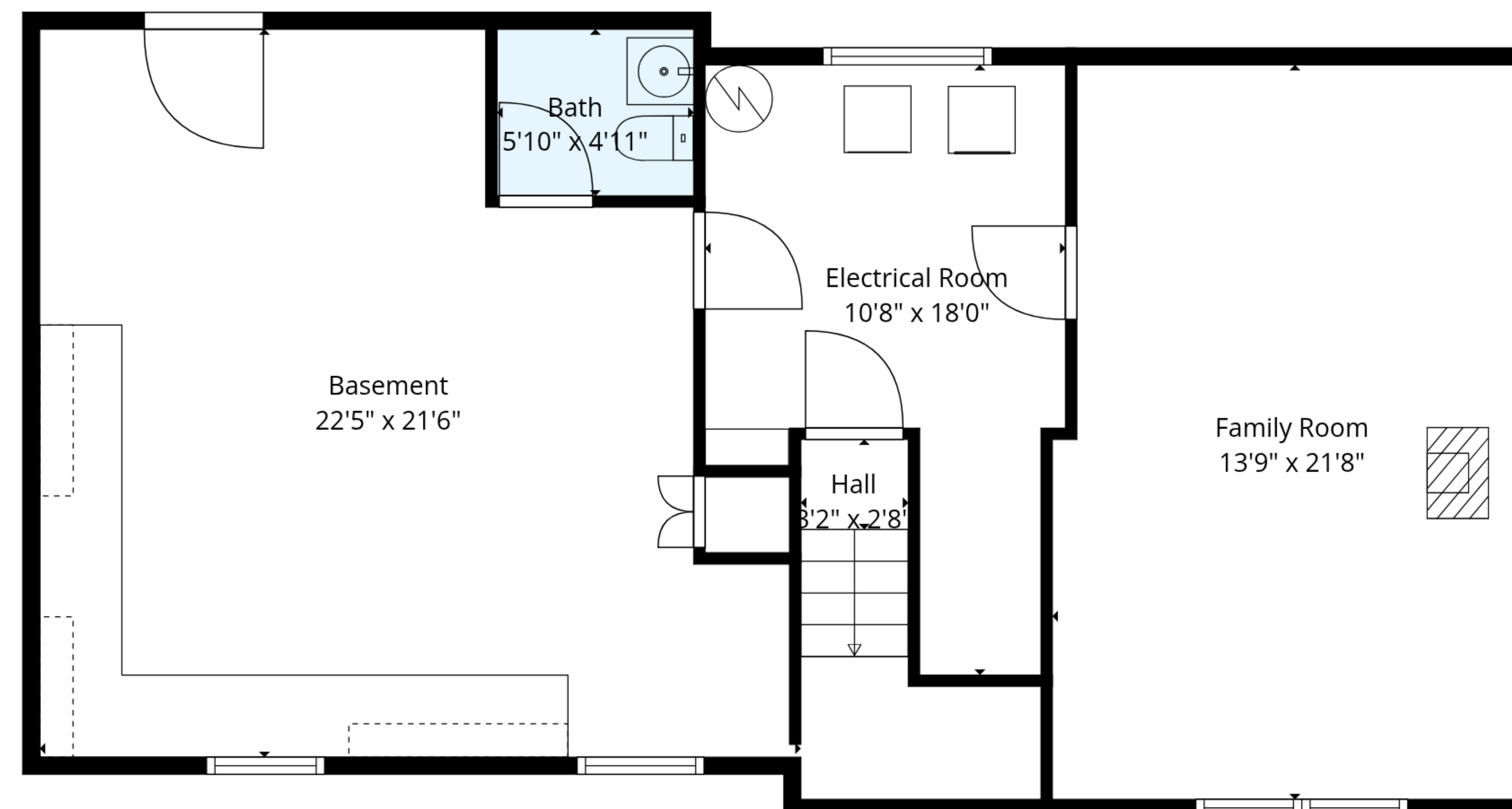
Floor 1
