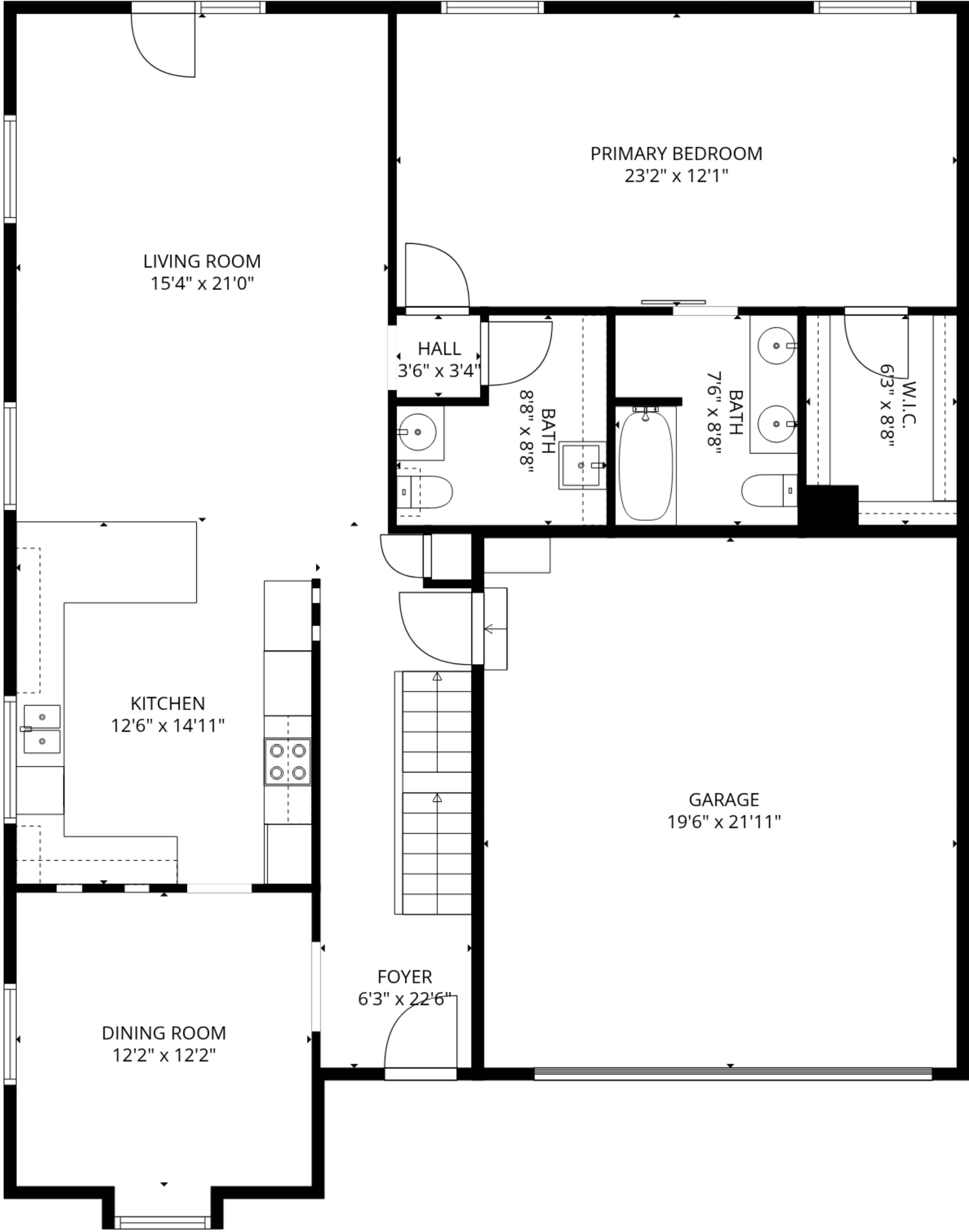
FLOOR 2
