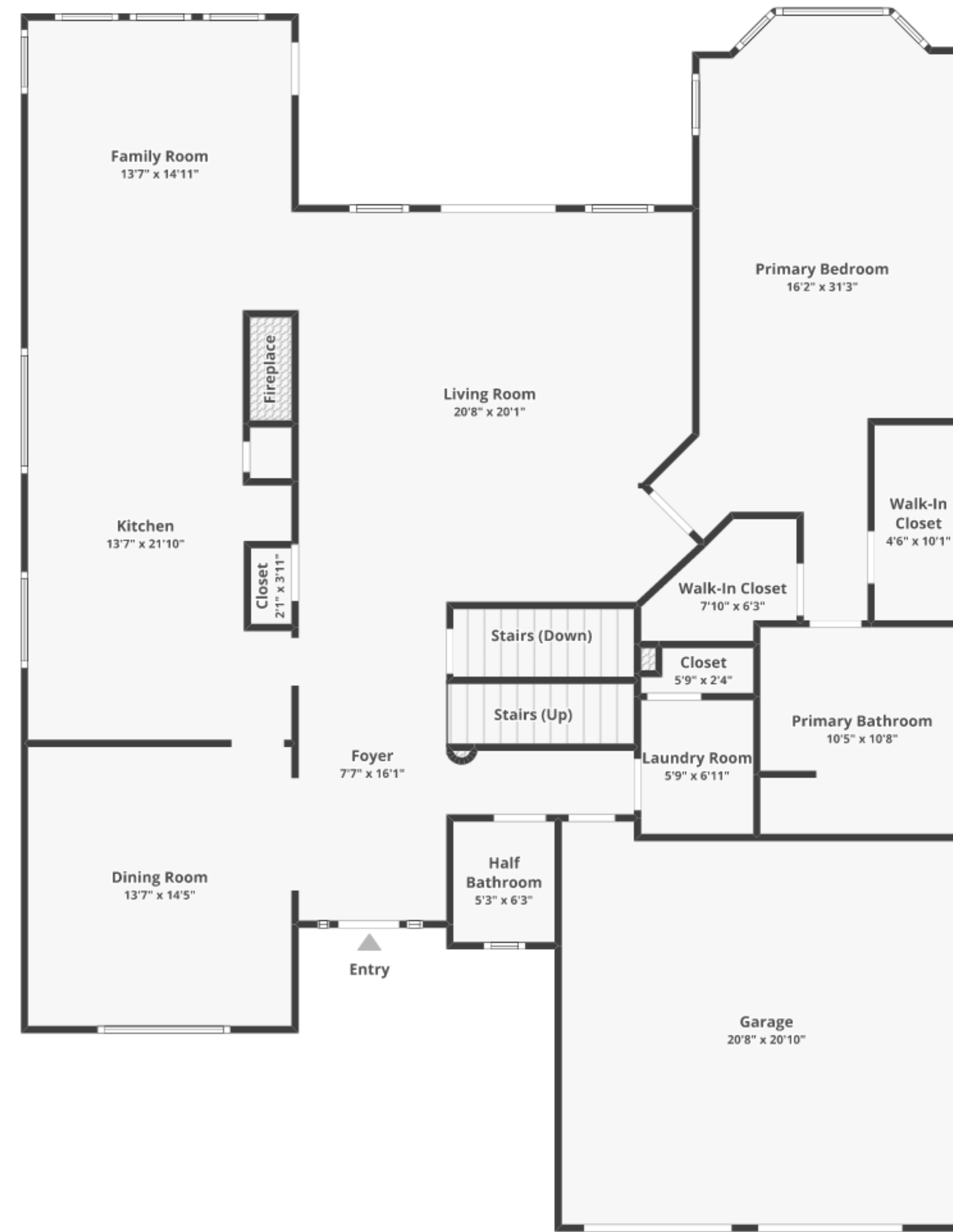
FLOOR 1 Finished area: ~1,907.14 sq. ft.
