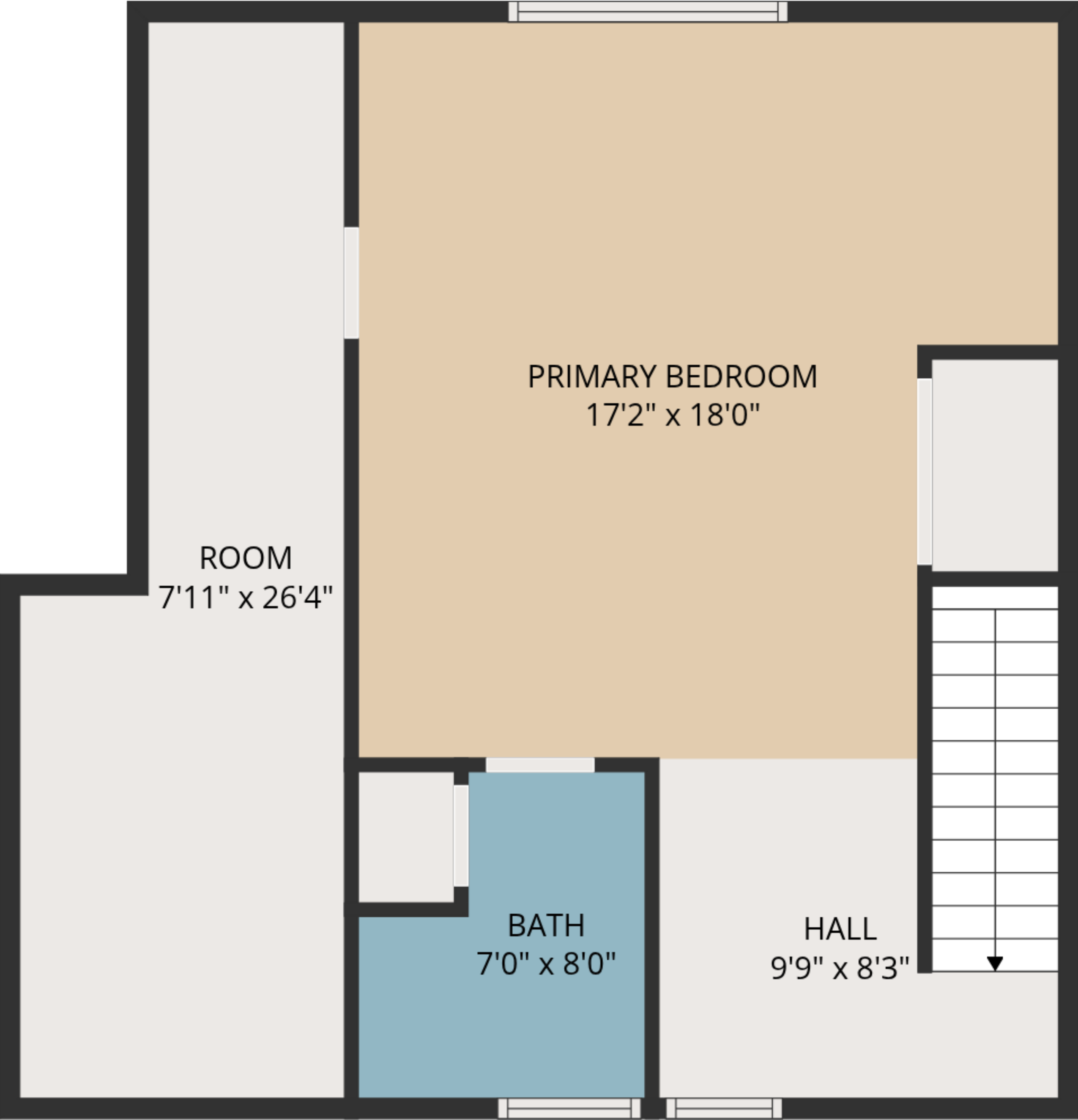
2ND FLOOR
