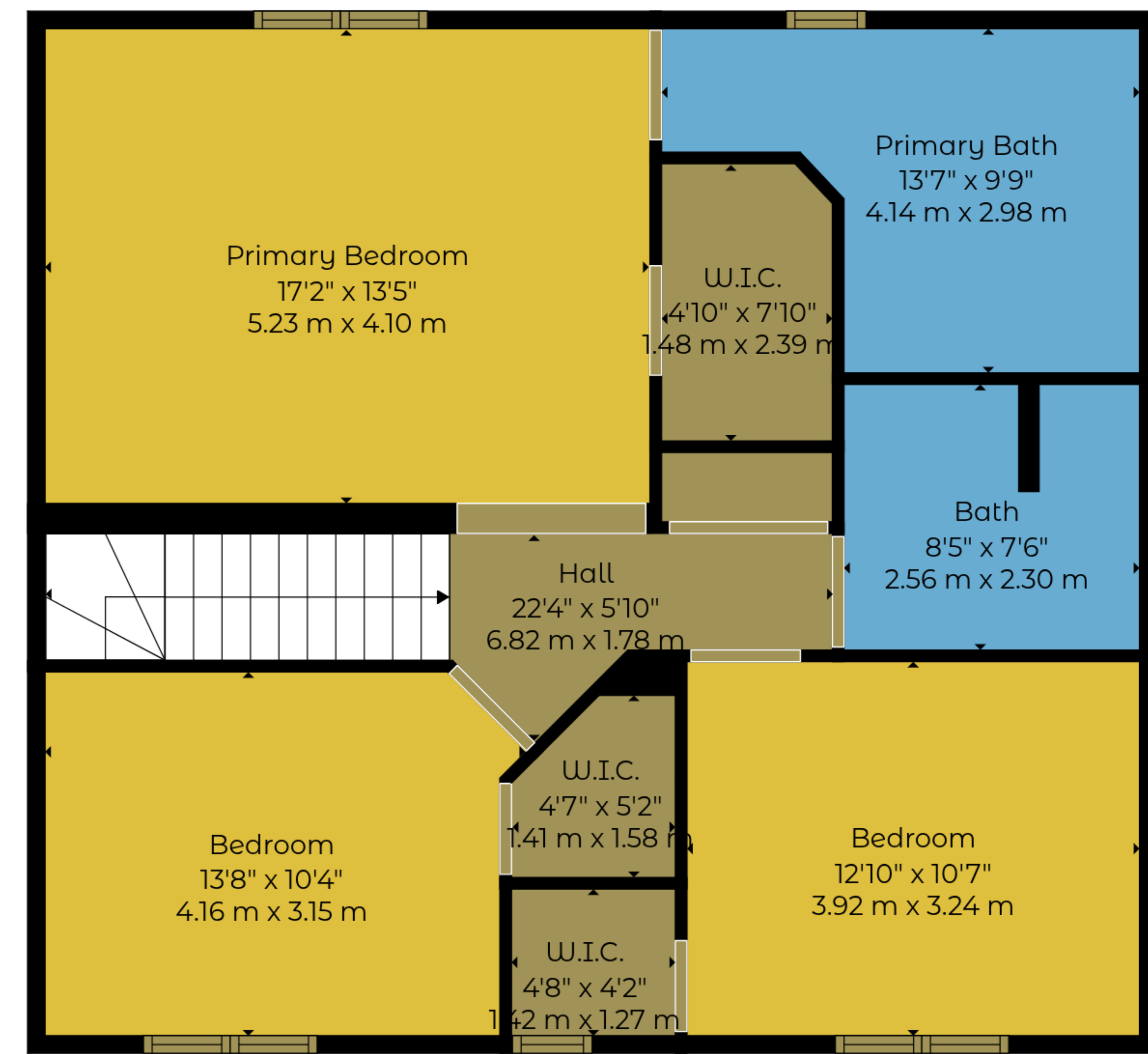
2nd Floor
