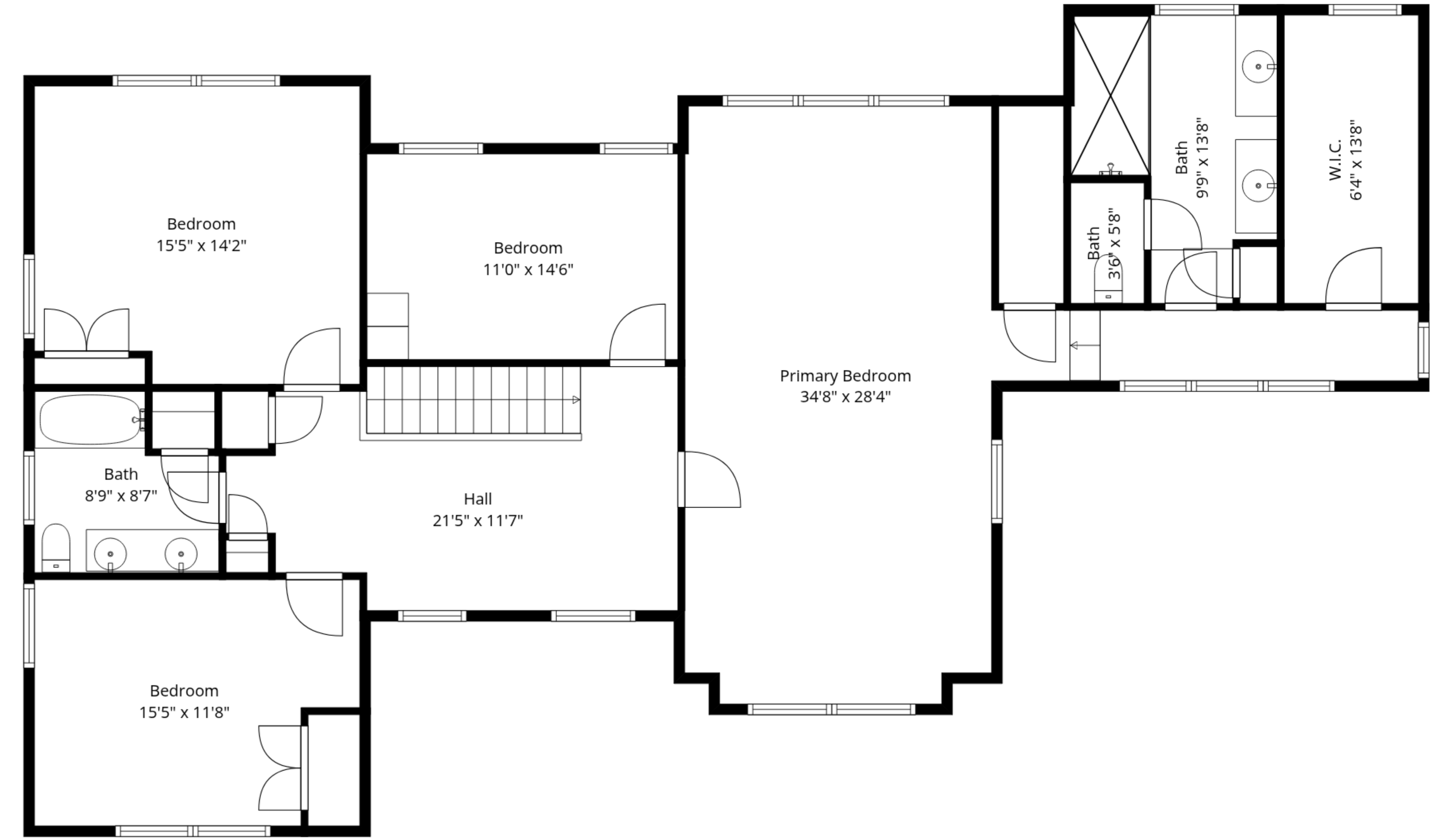
2nd Floor
