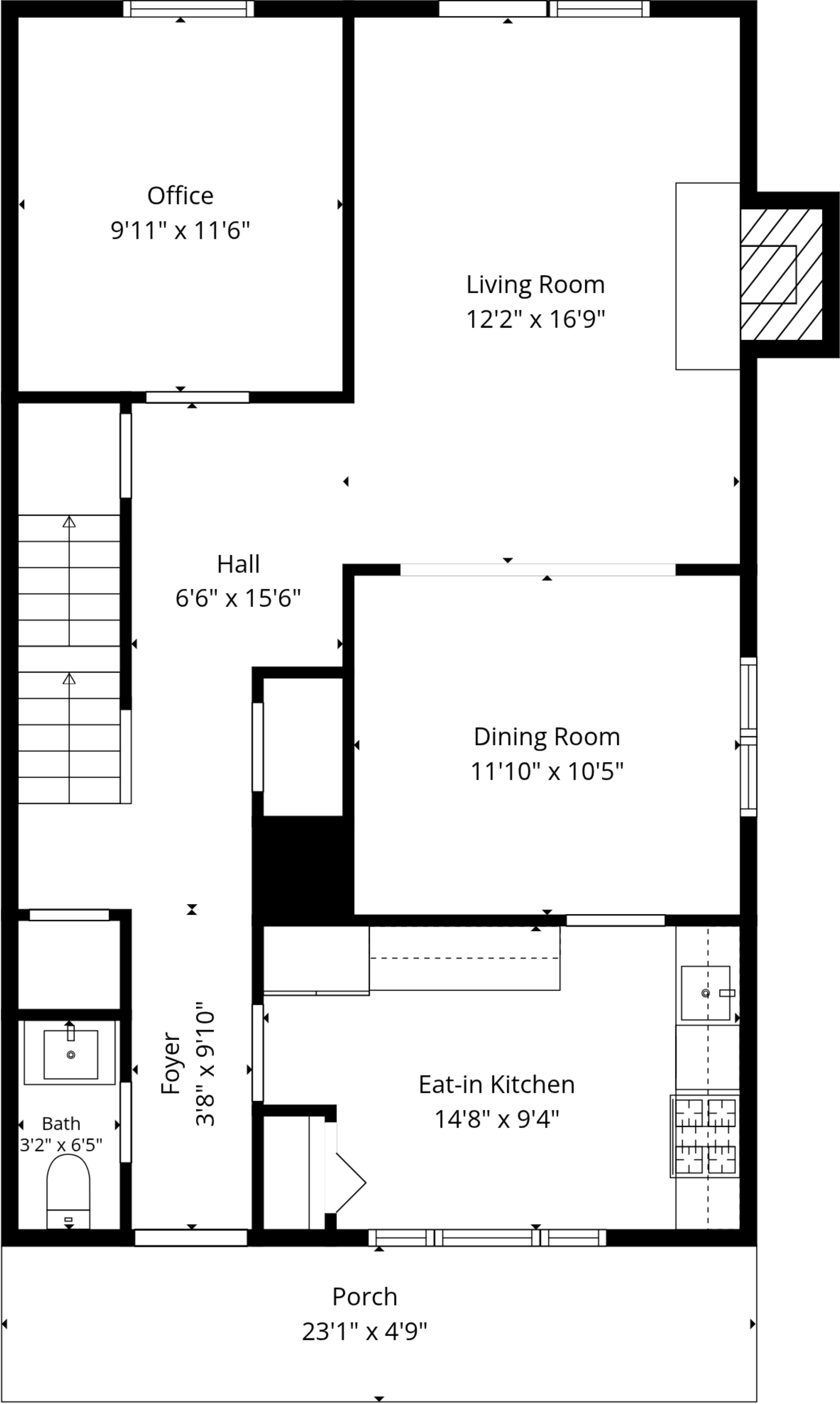
1st Floor
