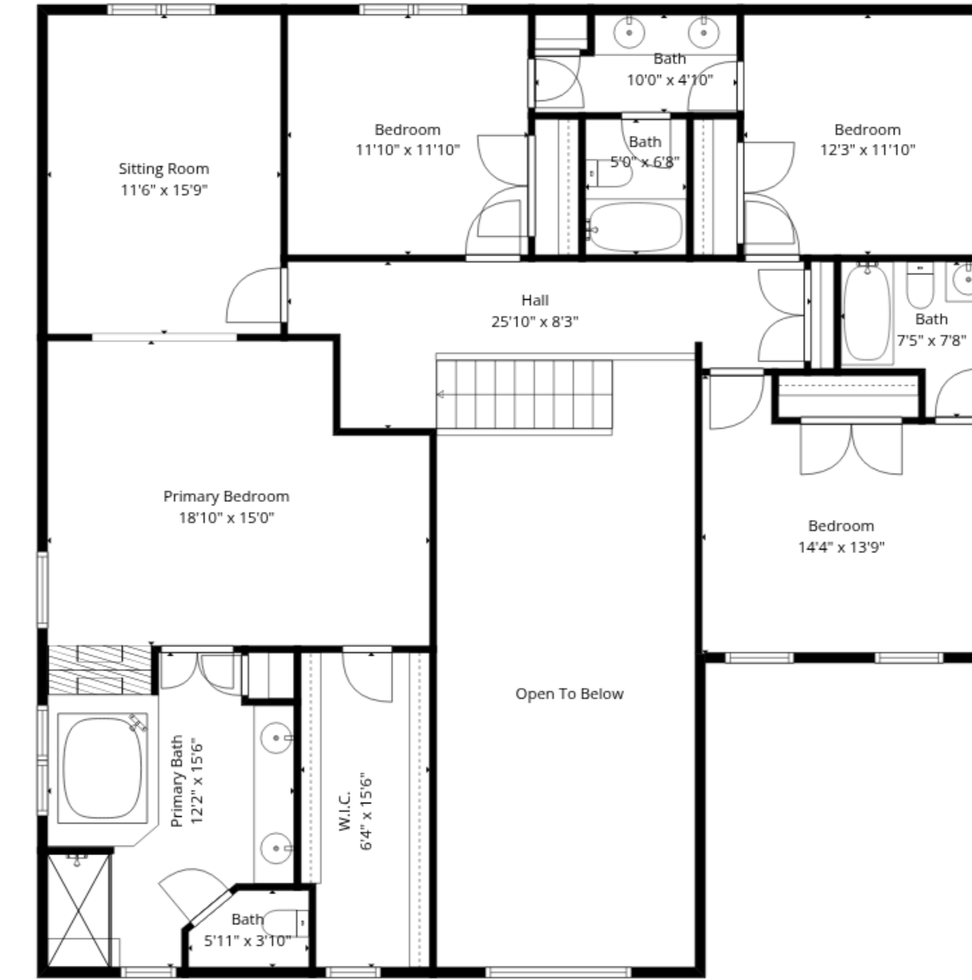
2nd Floor
