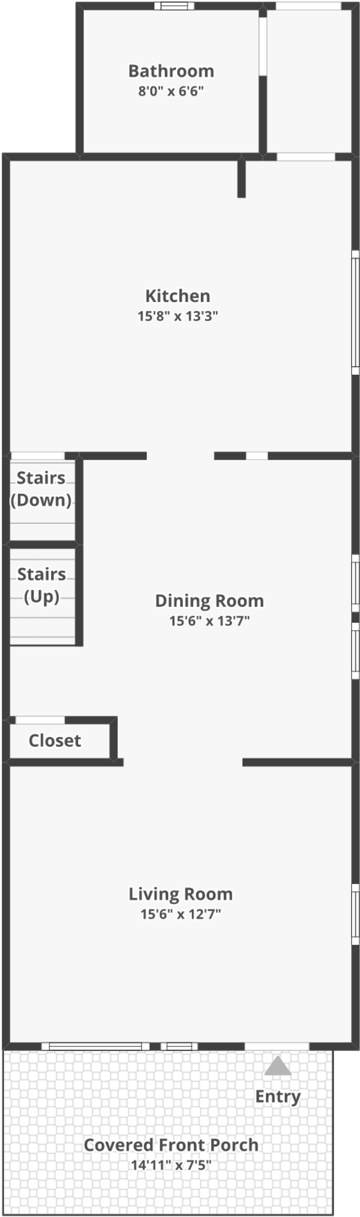
FLOOR 1
