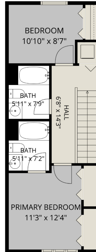
ABOVE MAIN
