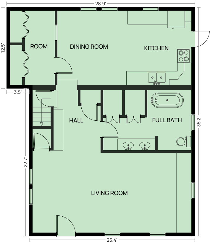
FIRST FLOOR Above grade · 8'1" ceiling · GLA 938 sq ft
