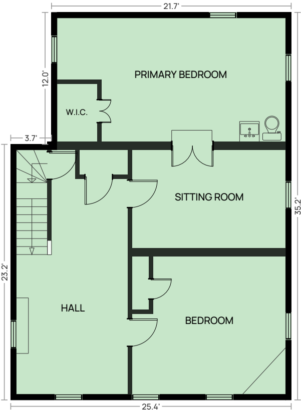
SECOND FLOOR Above grade · 8'10" ceiling · GLA 850 sq ft
