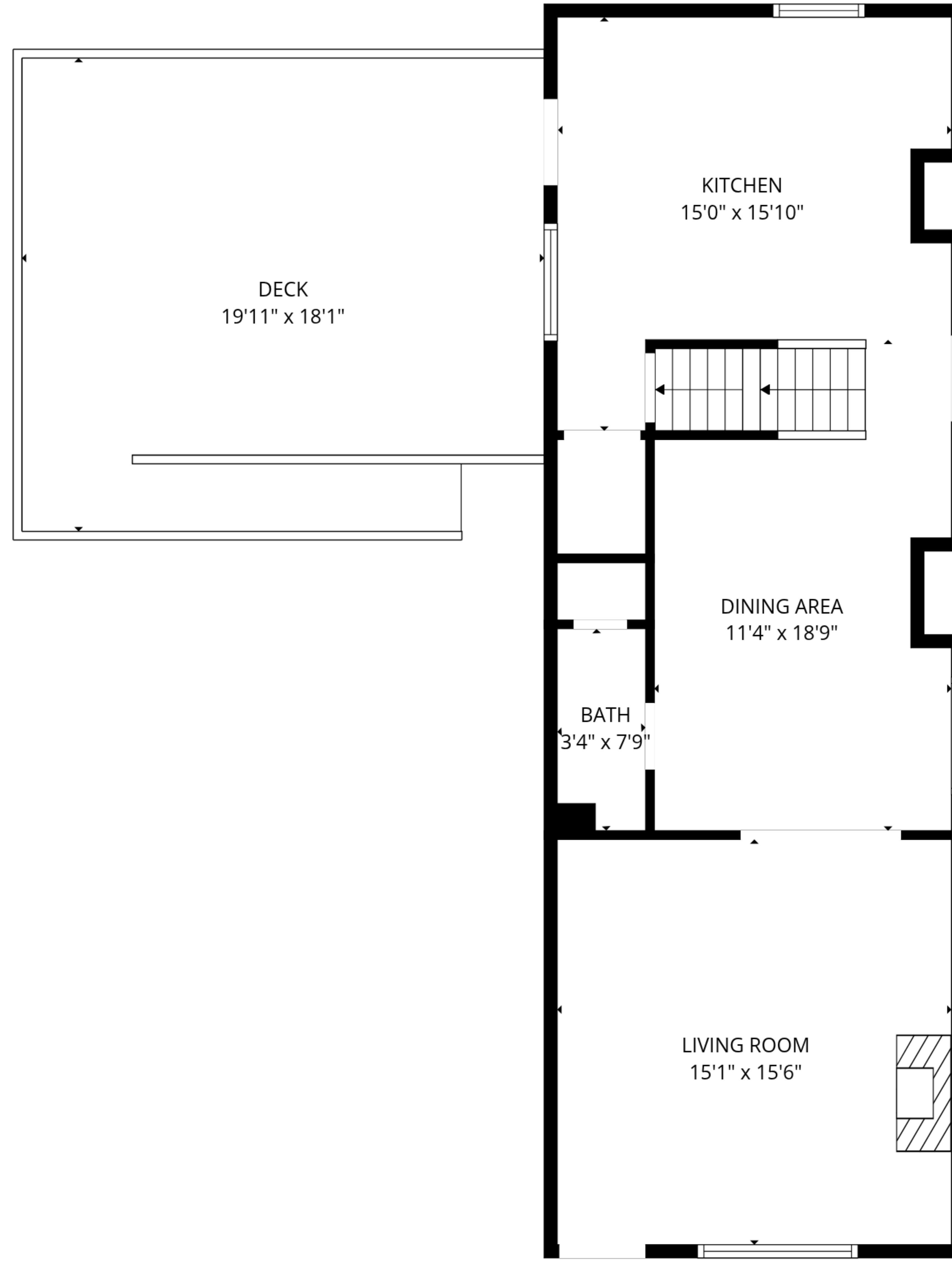
1st floor
