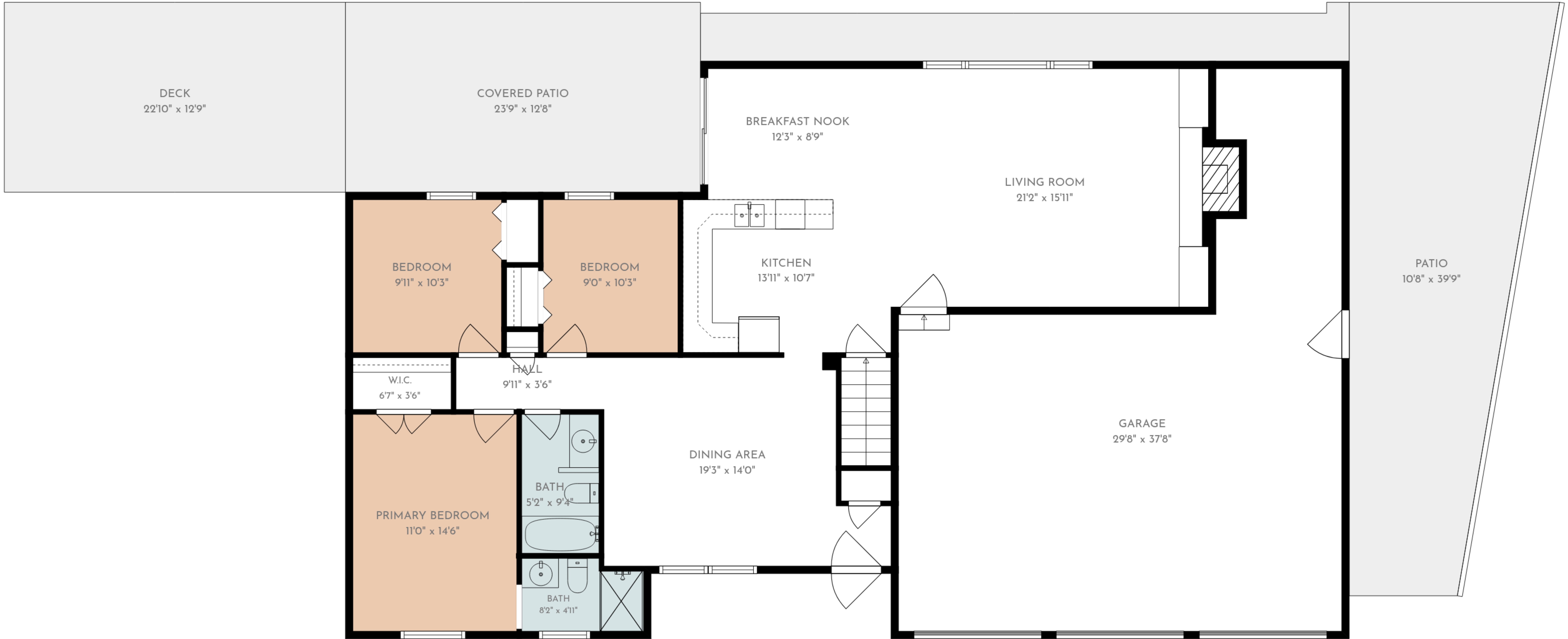
1st floor
