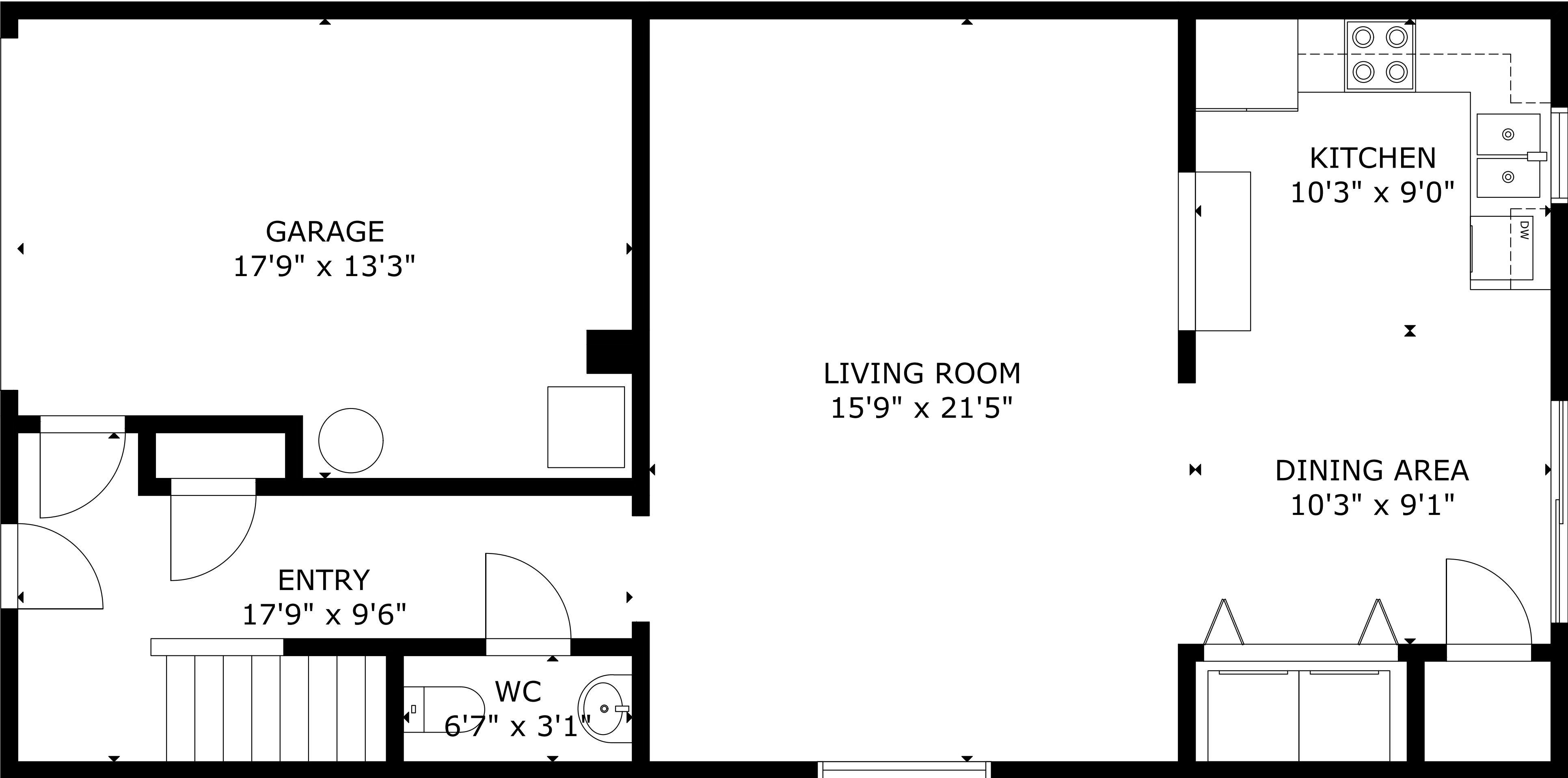
MAIN FLOOR
