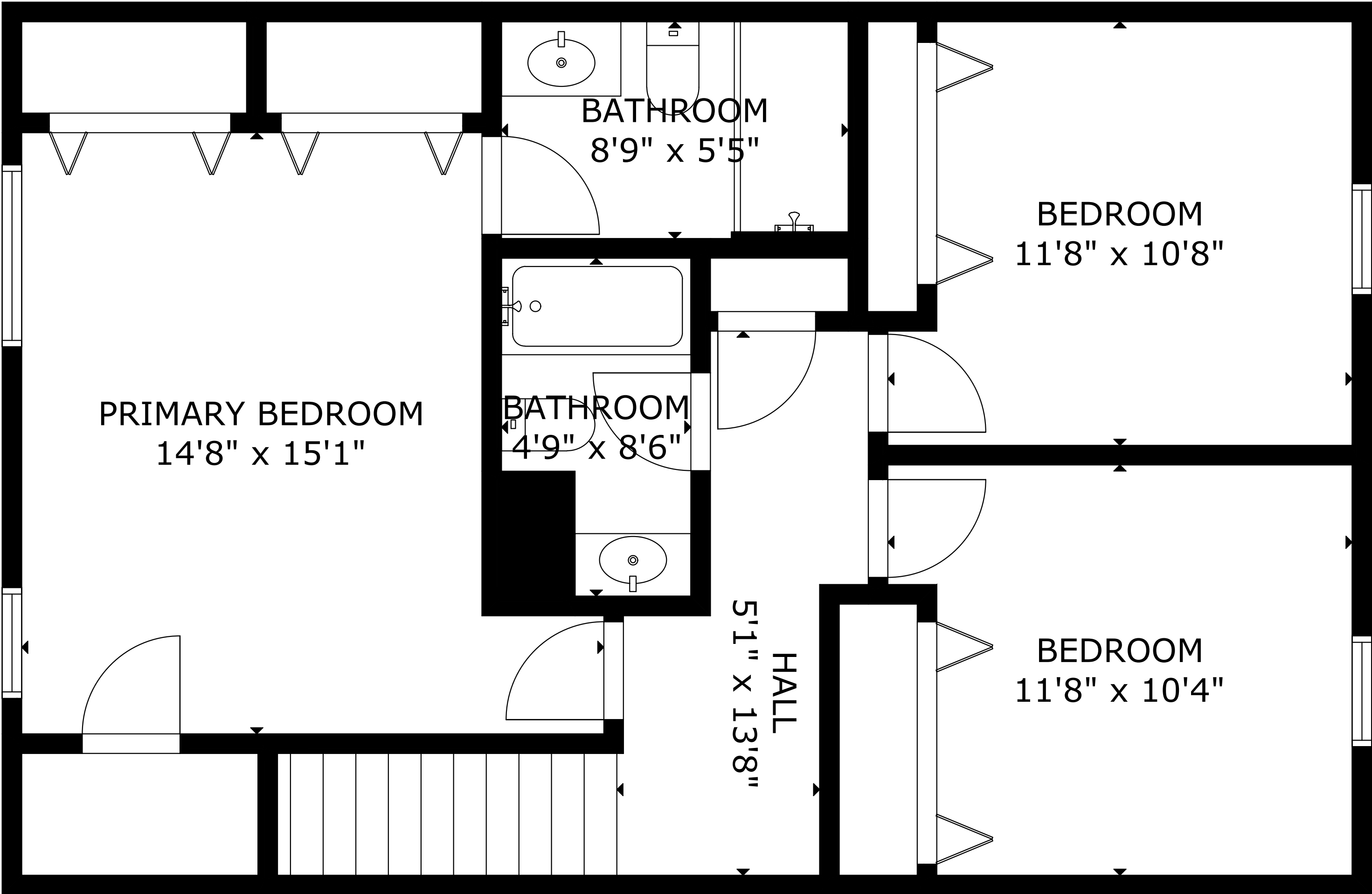
UPPER LEVEL 1
