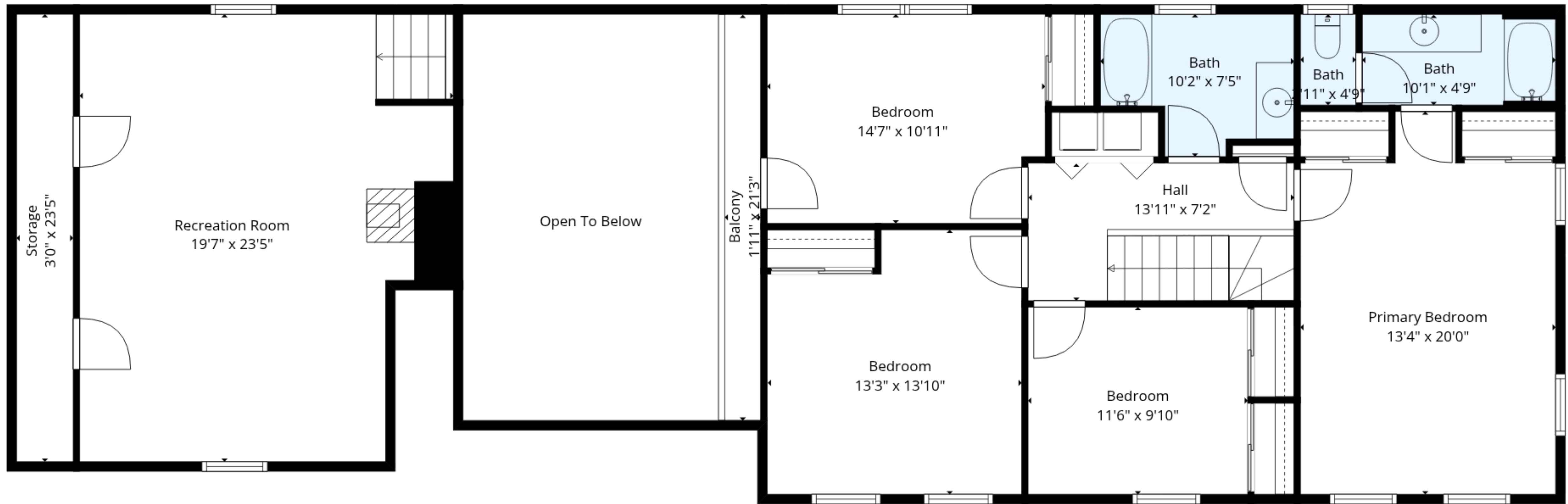
Floor 2
