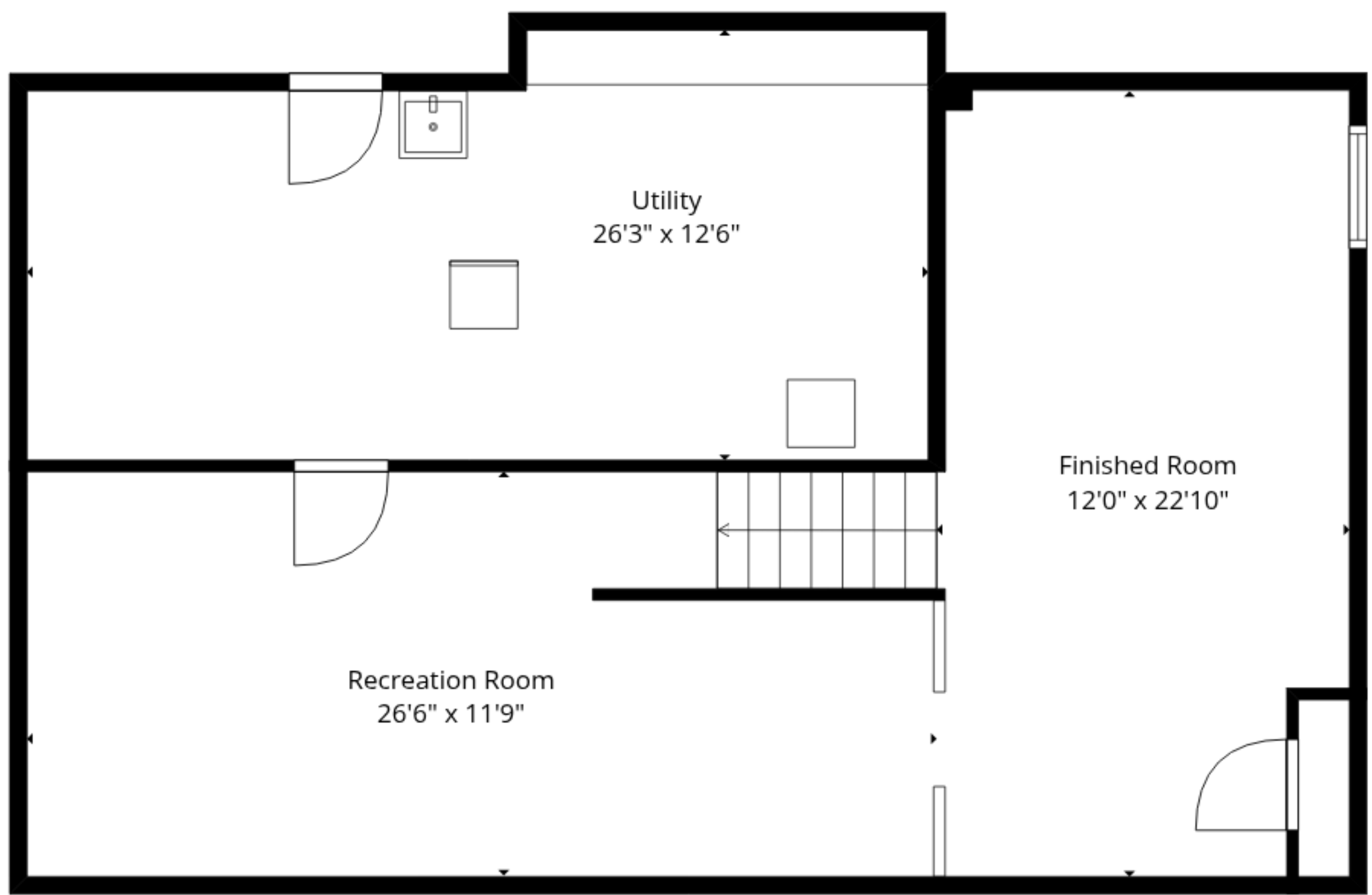
Basement
