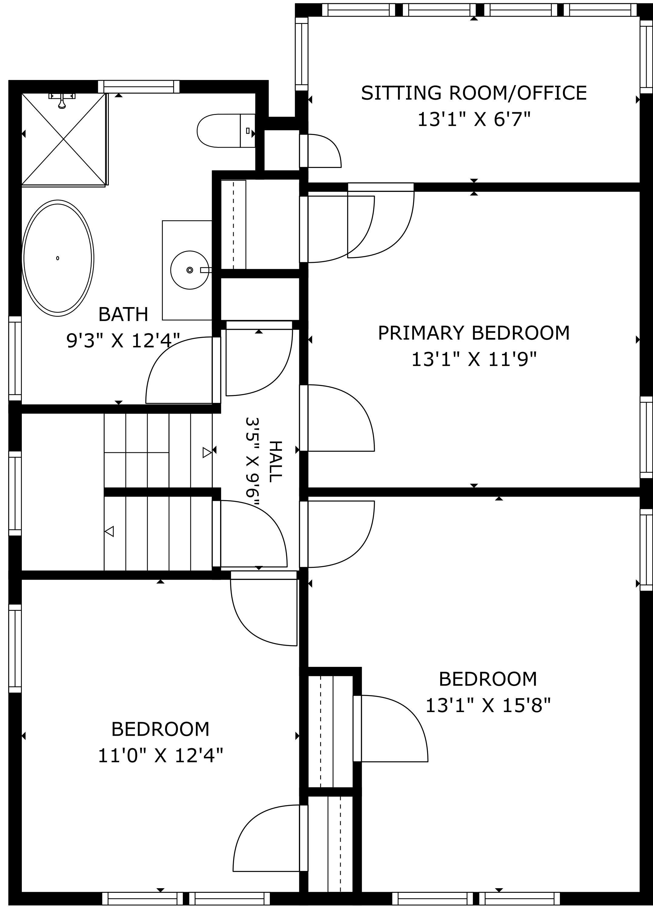
SECOND LEVEL
