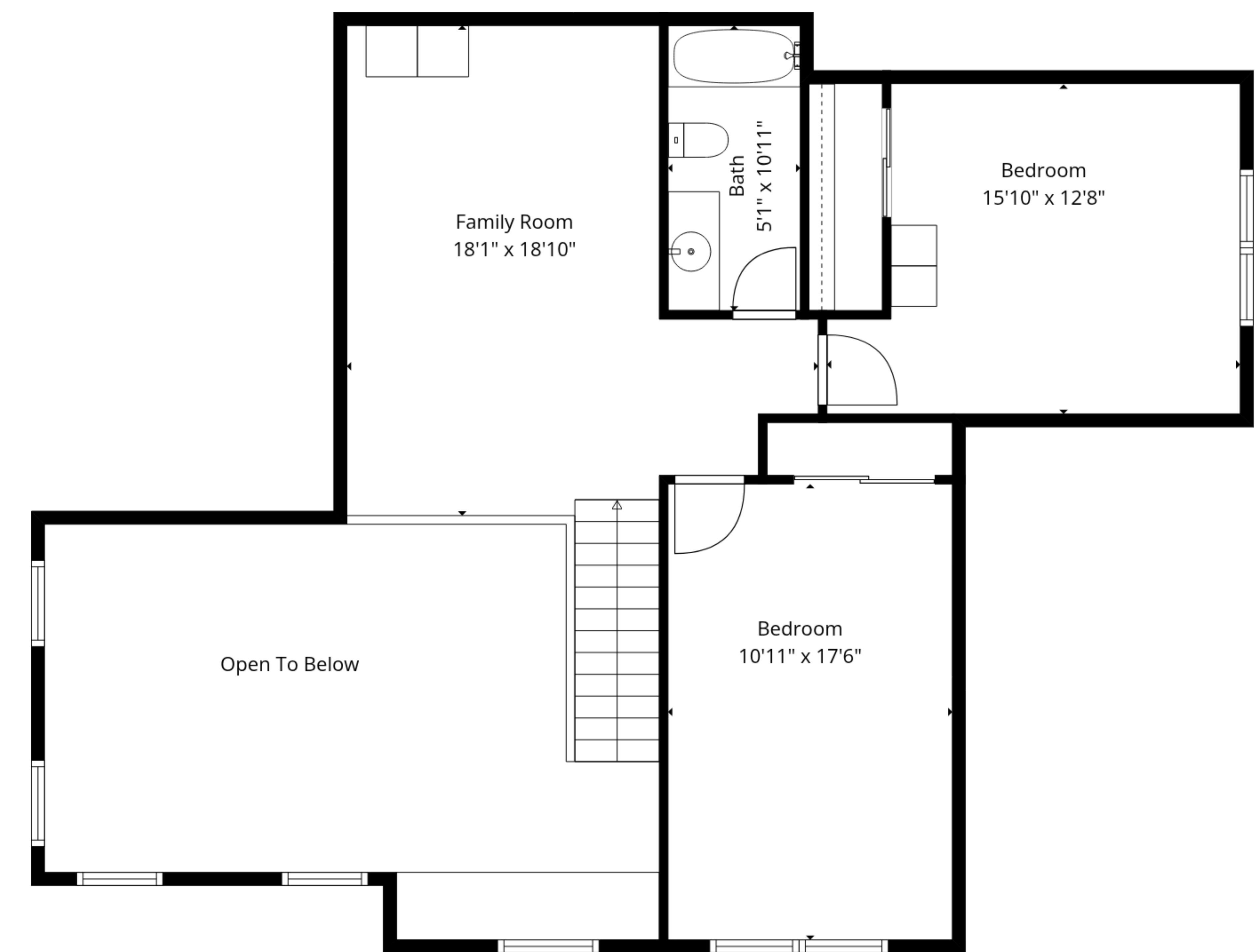
2nd Floor
