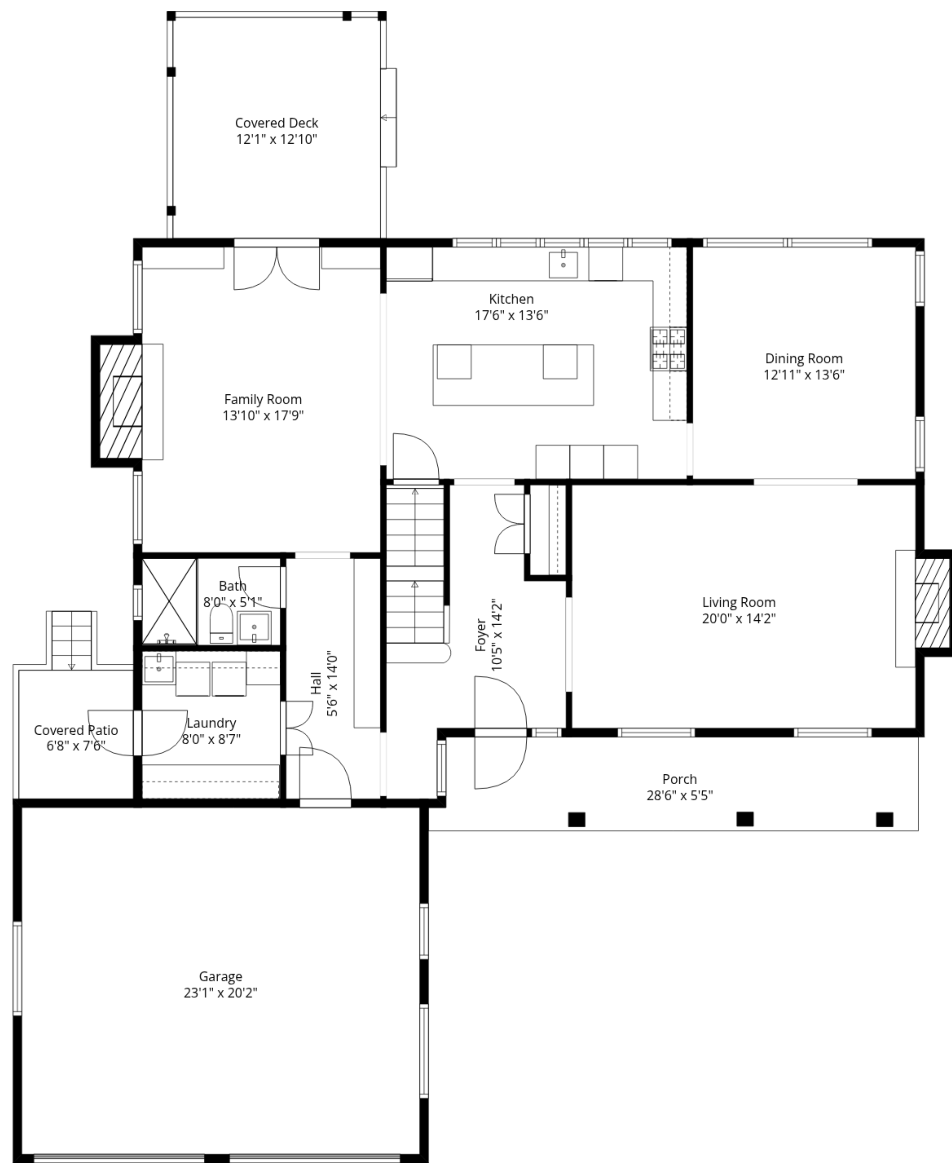
1st Floor
